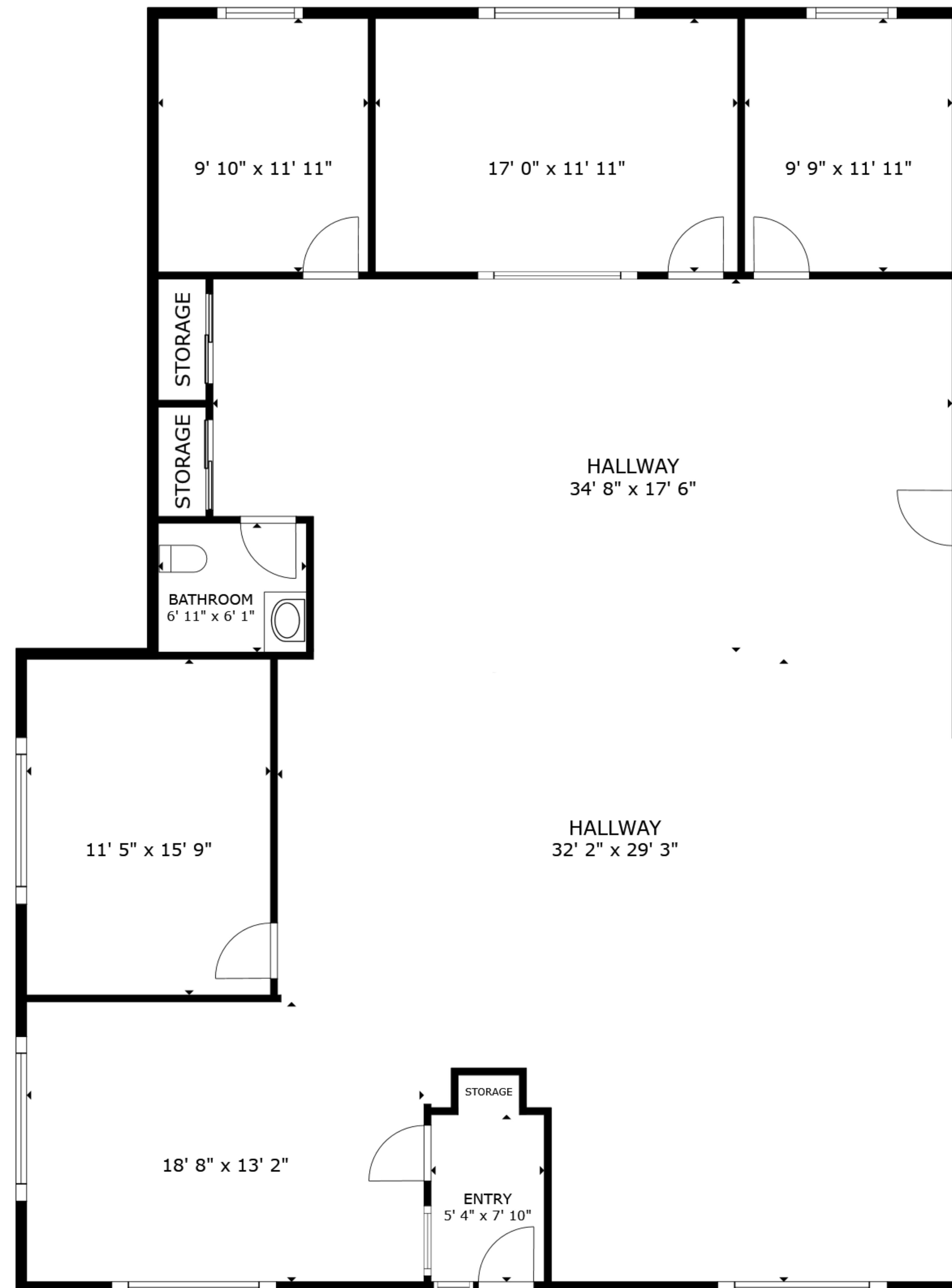
FLOOR PLAN
