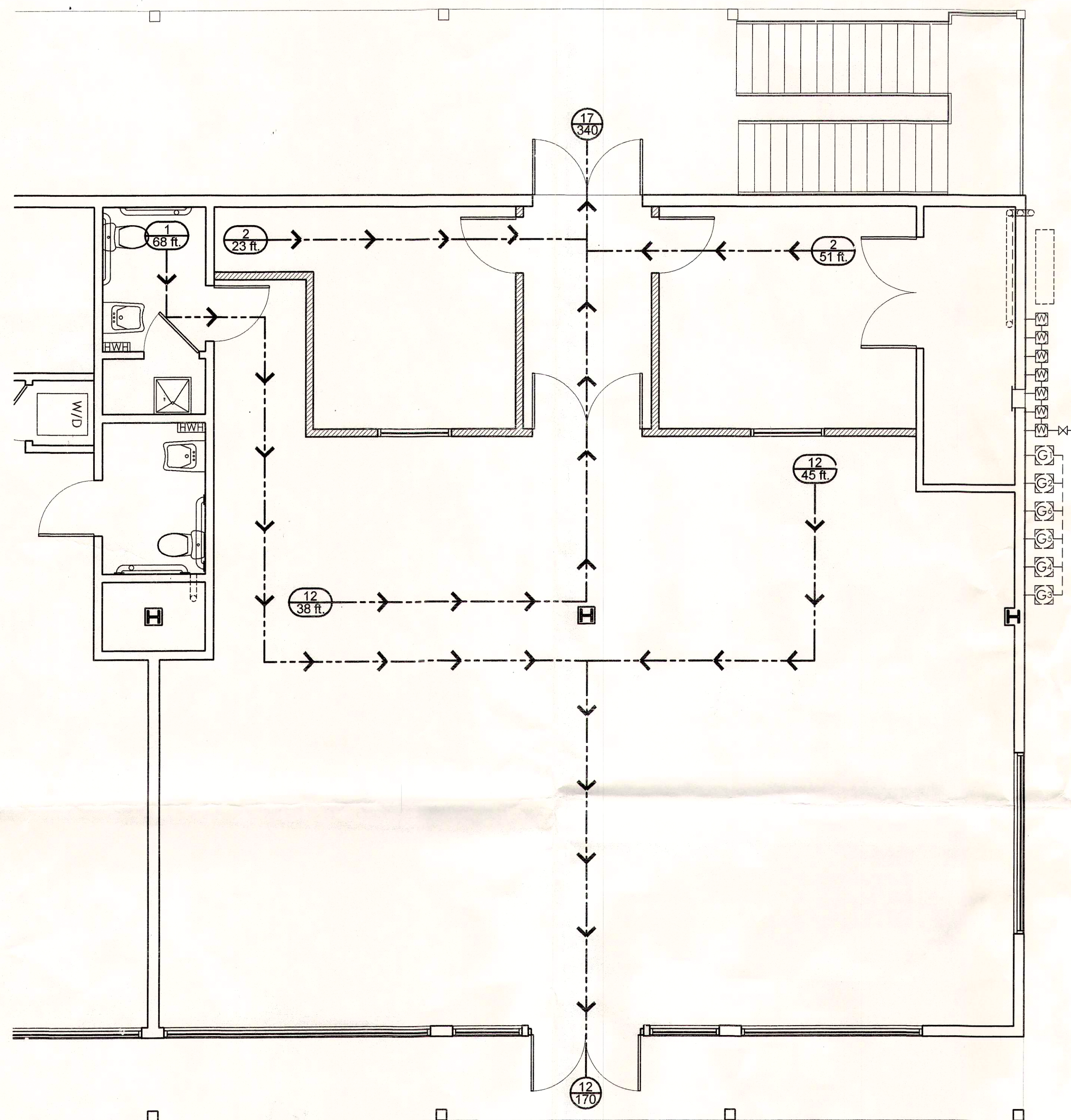
1 UNIT 2 EGRESS PLAN SCALE: 1/4" = 1'-0"
