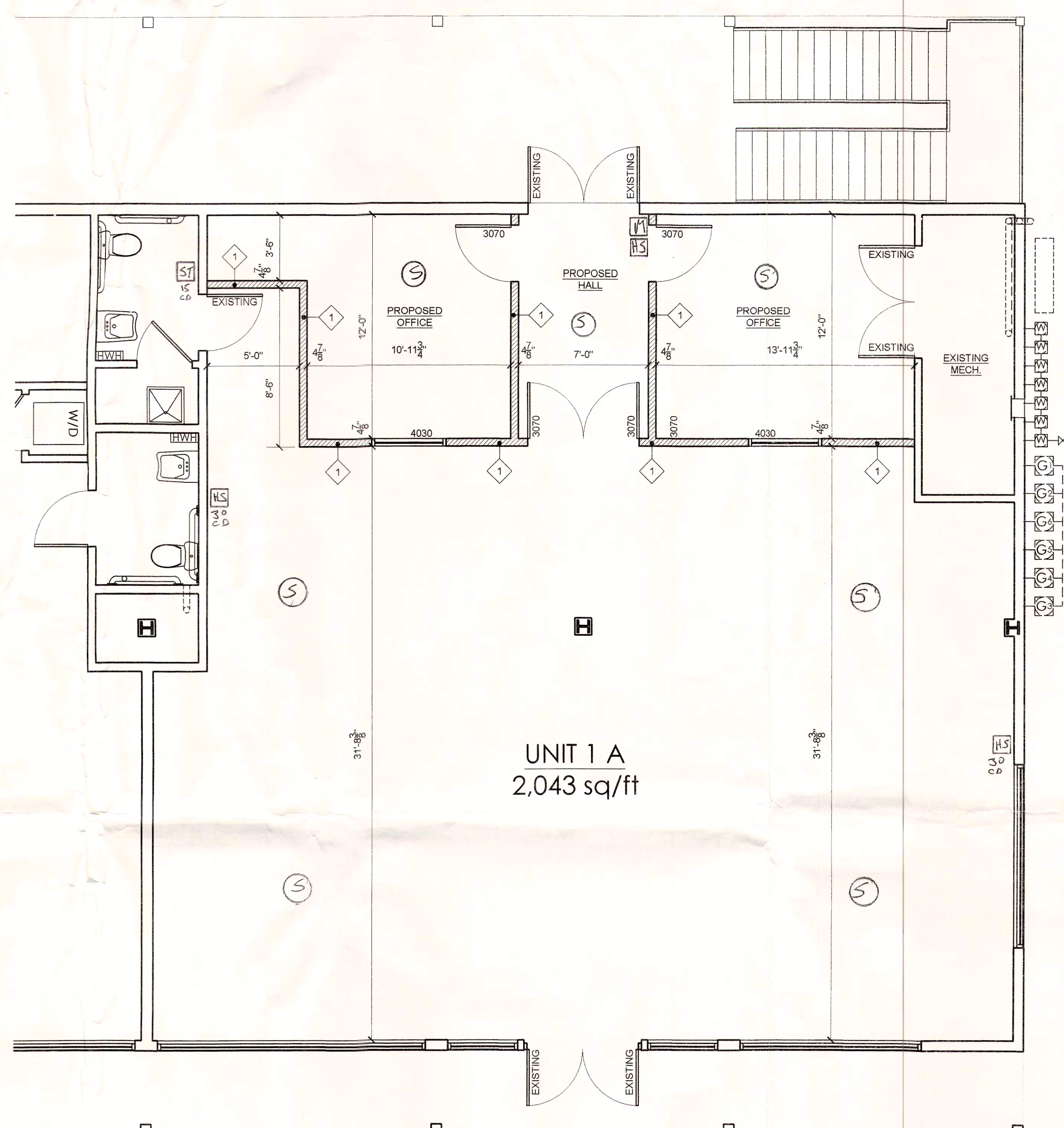
2 PROPOSED UNIT 1A FLOOR PLAN SCALE: 1/4" = 1'-0"
