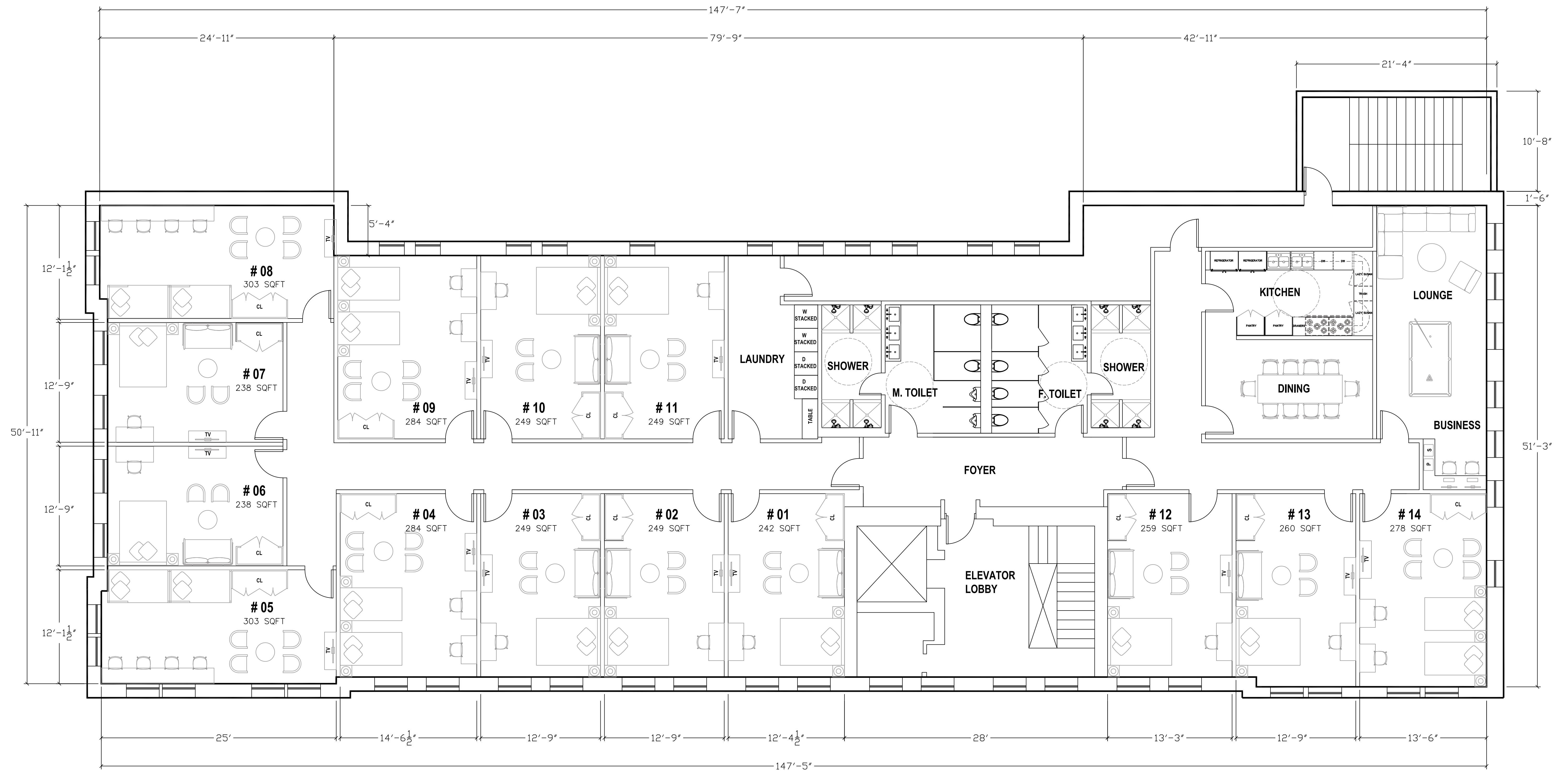
1 L4 FLOOR PLAN - OPT 2 3/16" = 1'-0"
