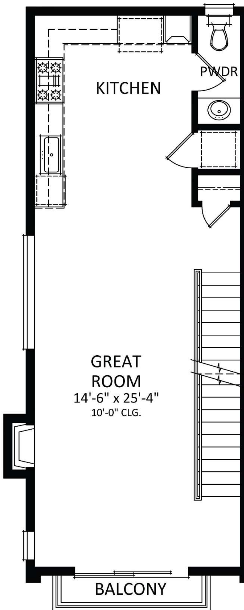
SECOND FLOOR
