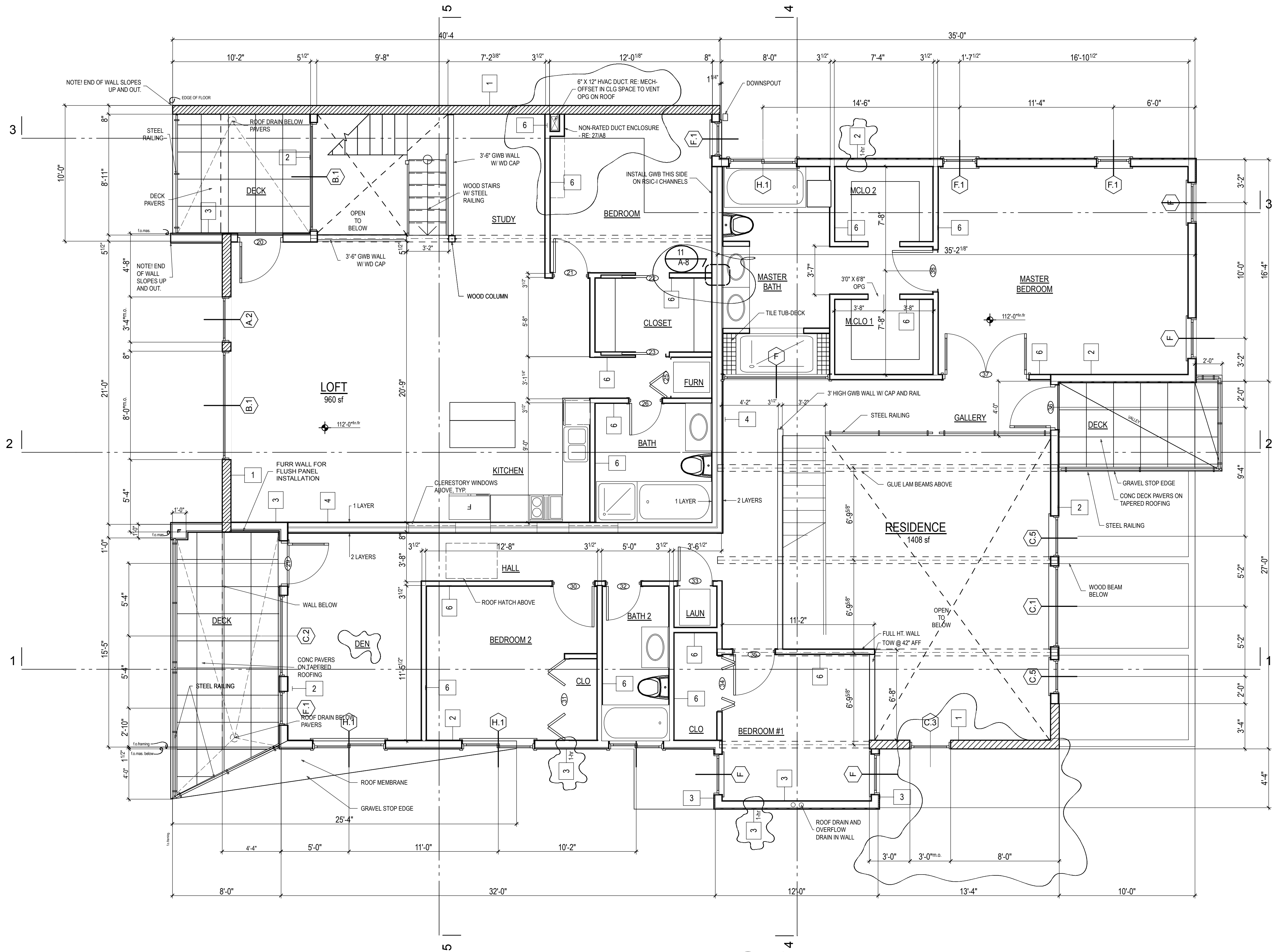
1 A-2 Second Floor Plan SCALE: 1/4" = 1'-0"
