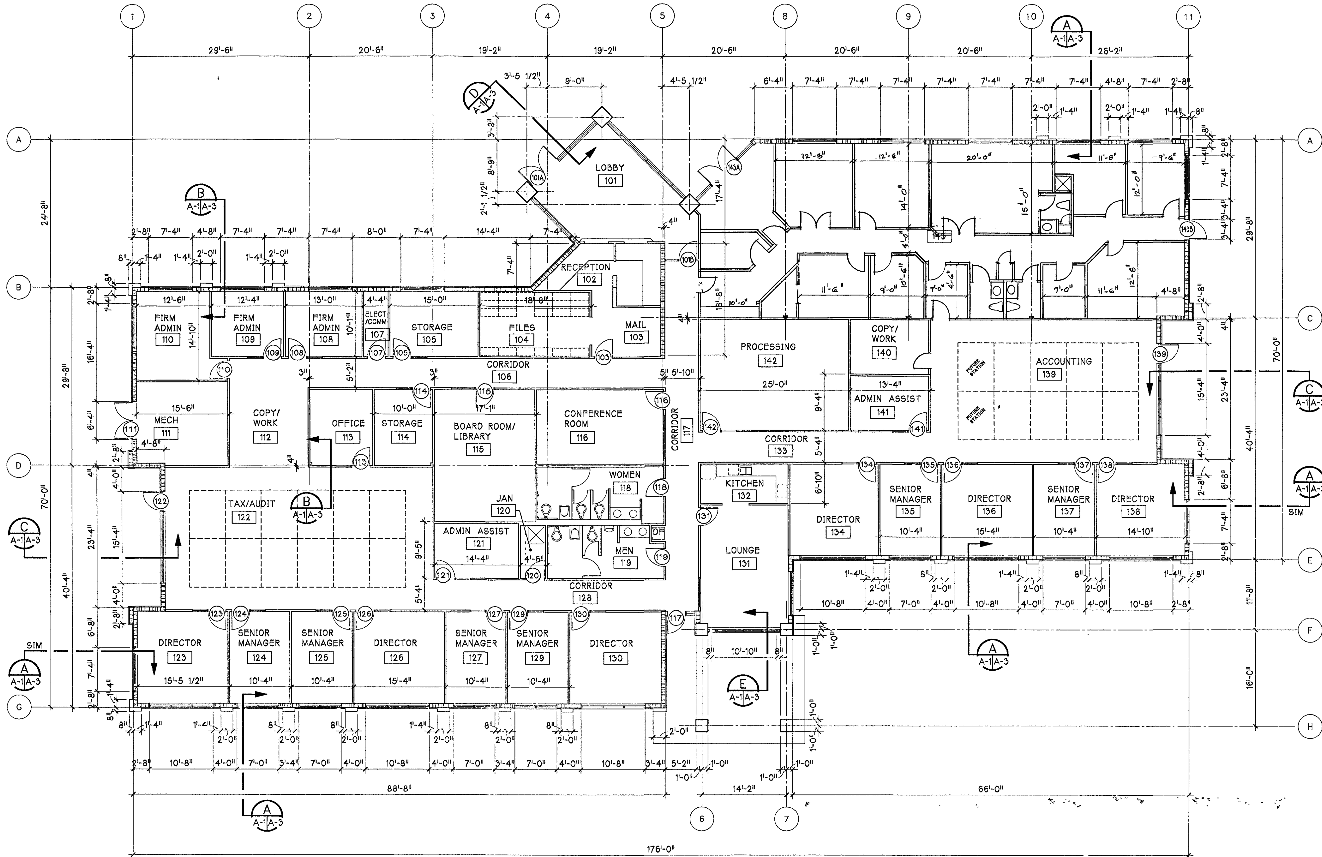
FLOOR PLAN 1/8" = 1'-0"
