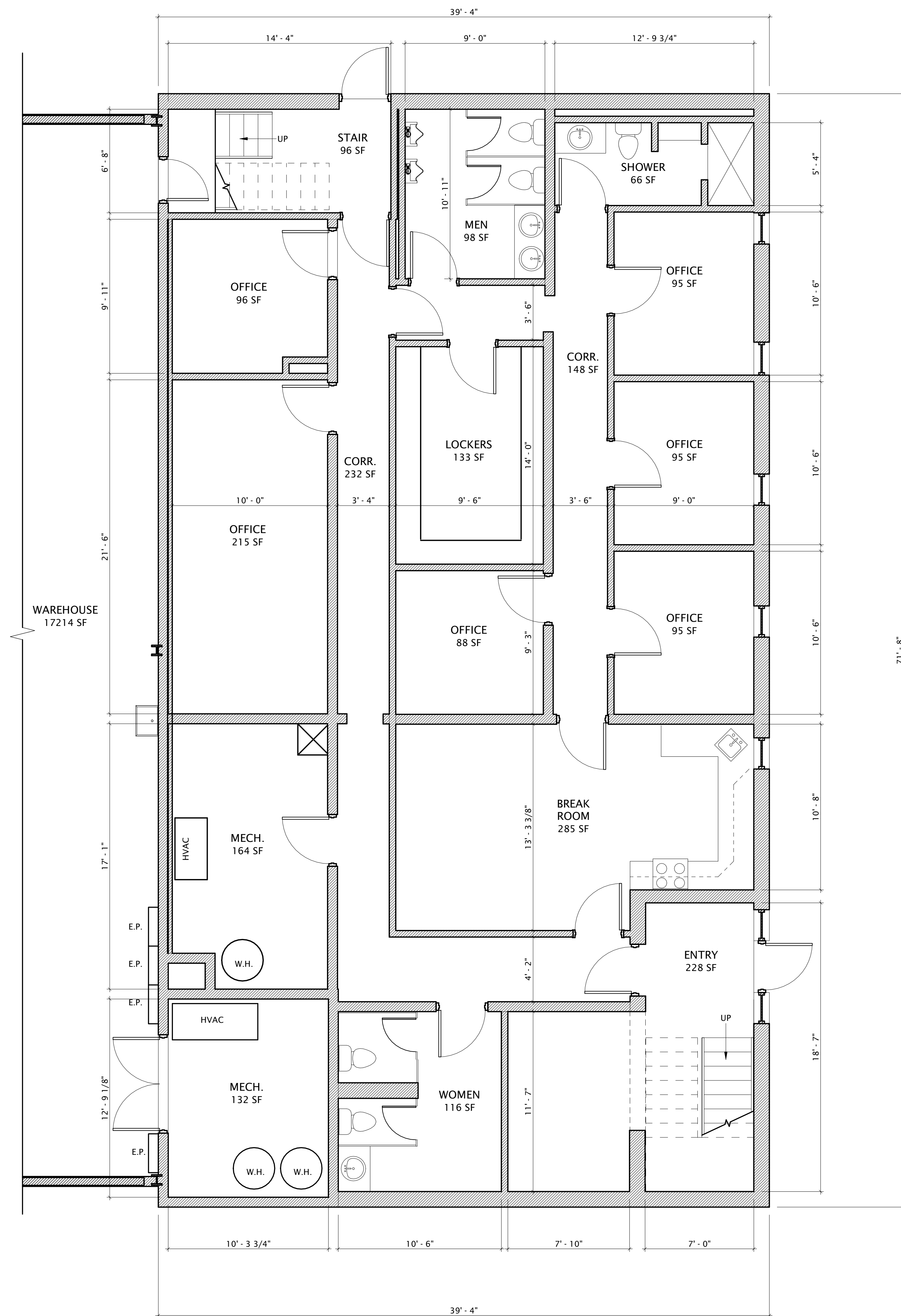
1 A2.0 GROUND FLOOR PLAN 1/4" = 1'-0"
