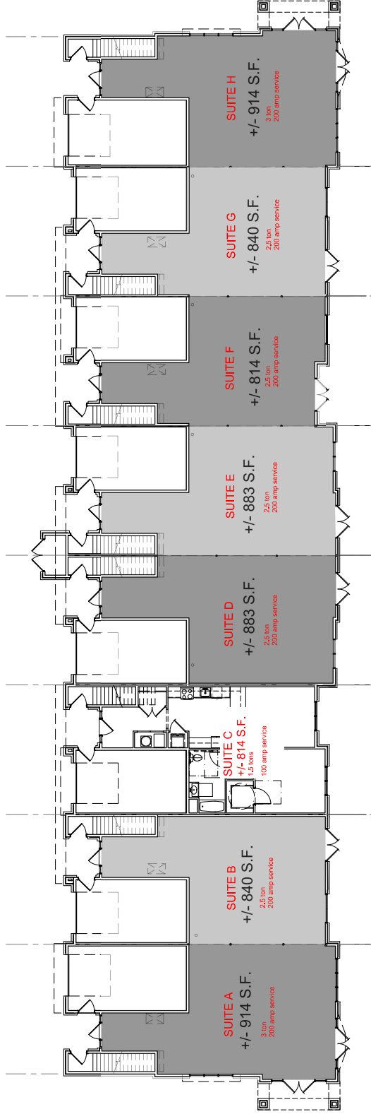
1 GROUND FLOOR PLAN - BUILDING 5 Scale: 1/8" = 1'-0"
