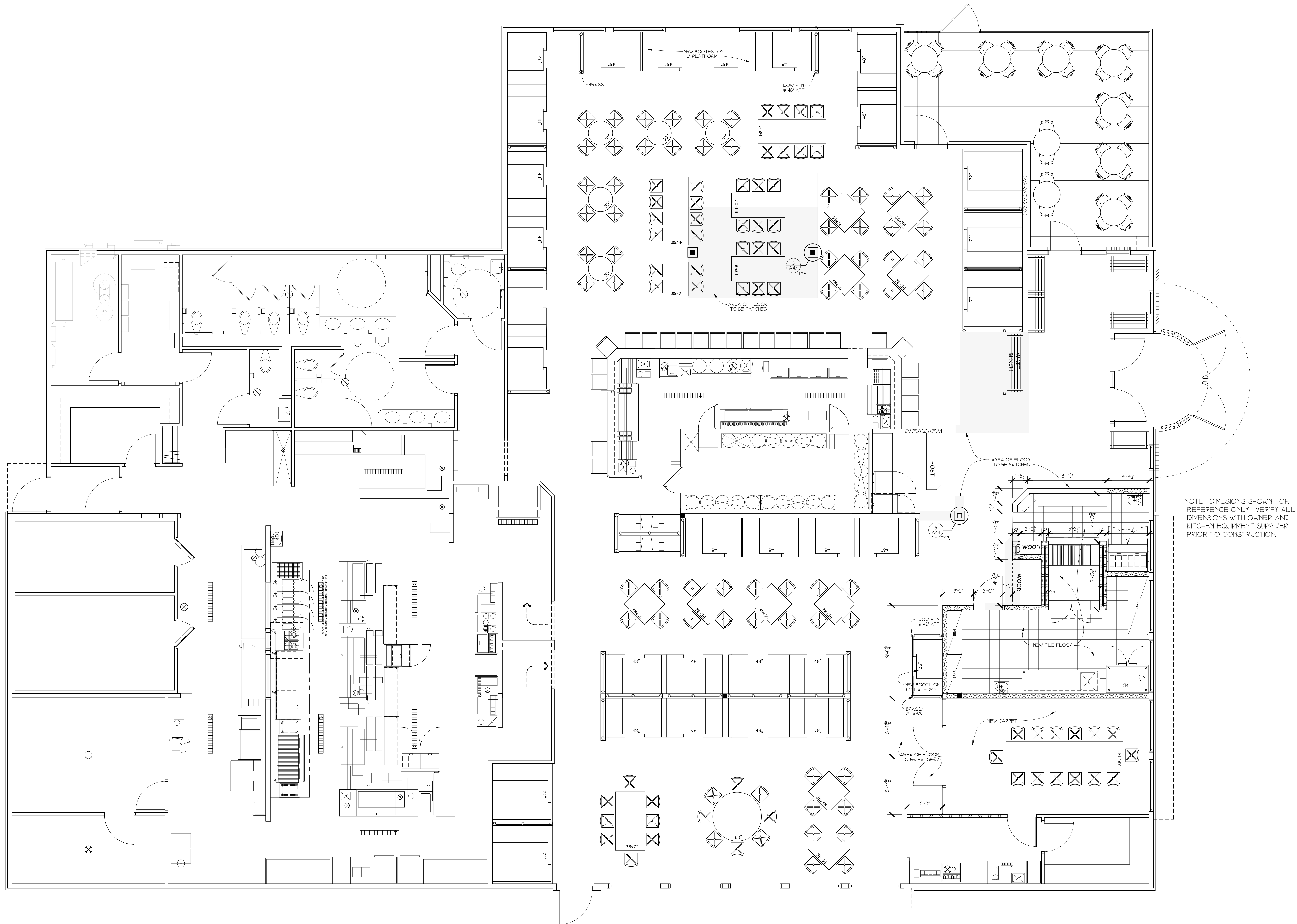
DEMO FLOOR PLAN 1/4" = 1'-0"
