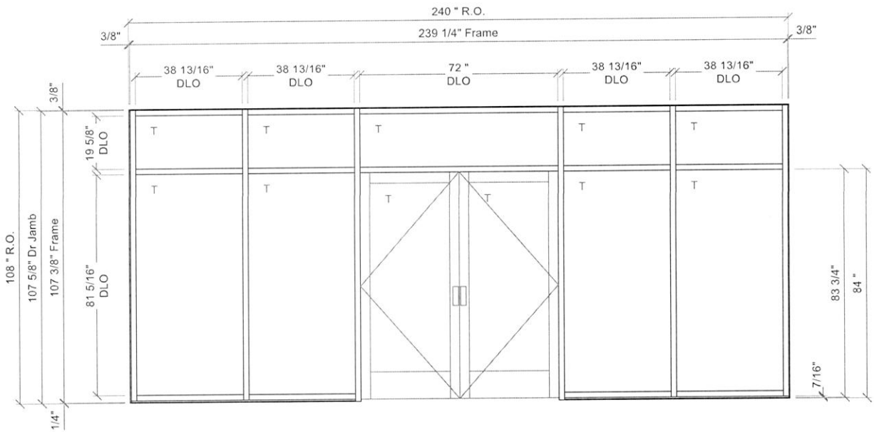
LW - Misc - 1 - 001 - SF1 (1 Thus) Frame: (Clear) YES 45 TU : Storefront : Screw Spline : Thermal : Center Set : Outside Glaze
