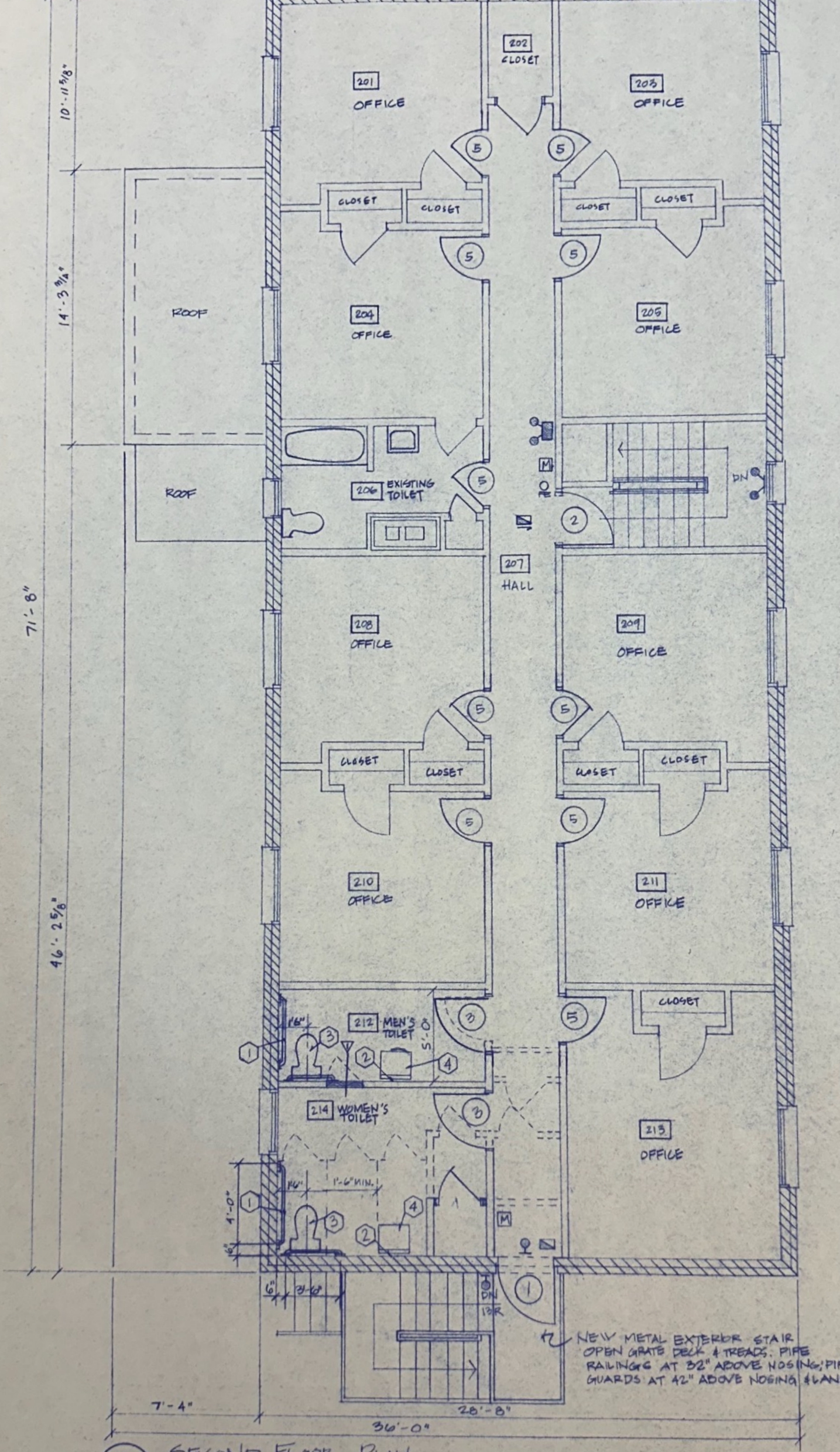
3 SECOND FLOOR PLAN A1.3 1/4" = 1'-0"
