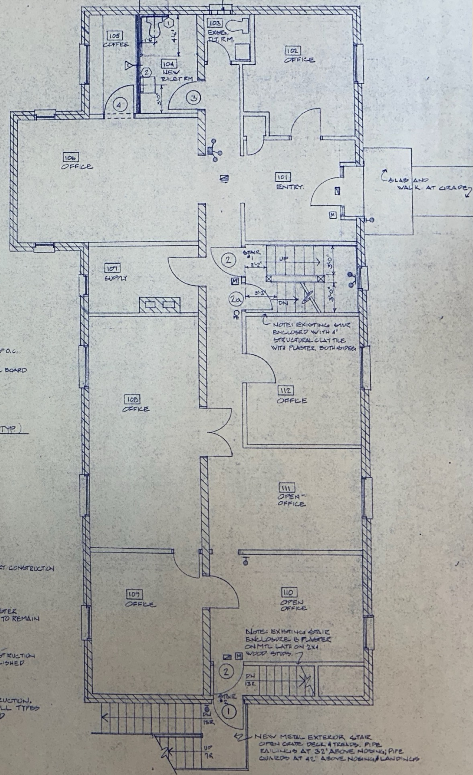
2 FIRST FLOOR PLAN A1.2 1/4" = 1'-0"
