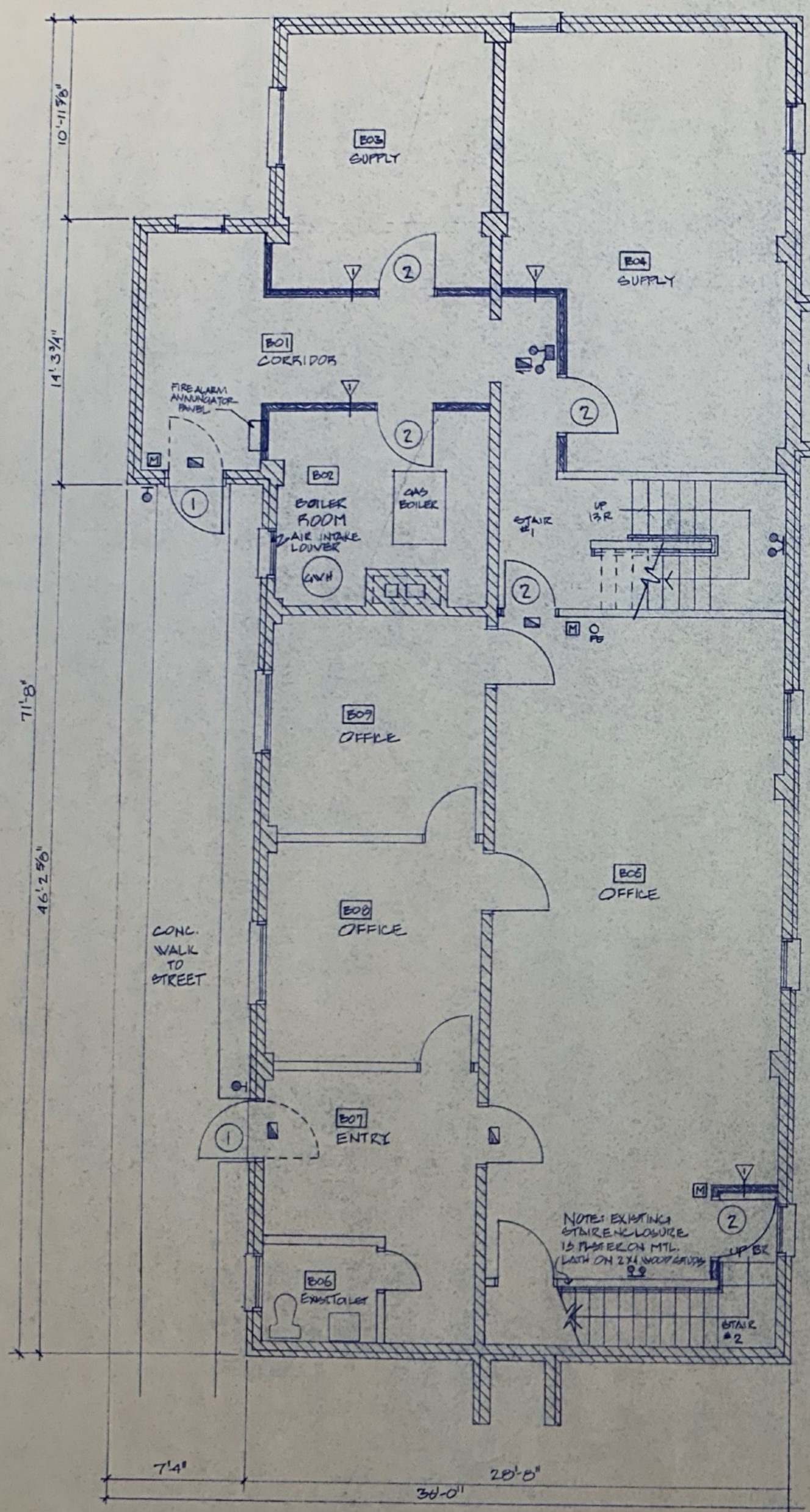
1 LOWER LEVEL PLAN A1.2 1/4" = 1'-0"
