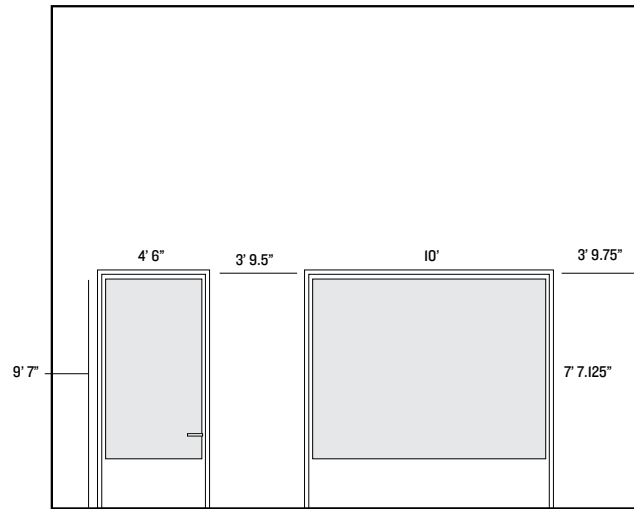
Exterior—Front
