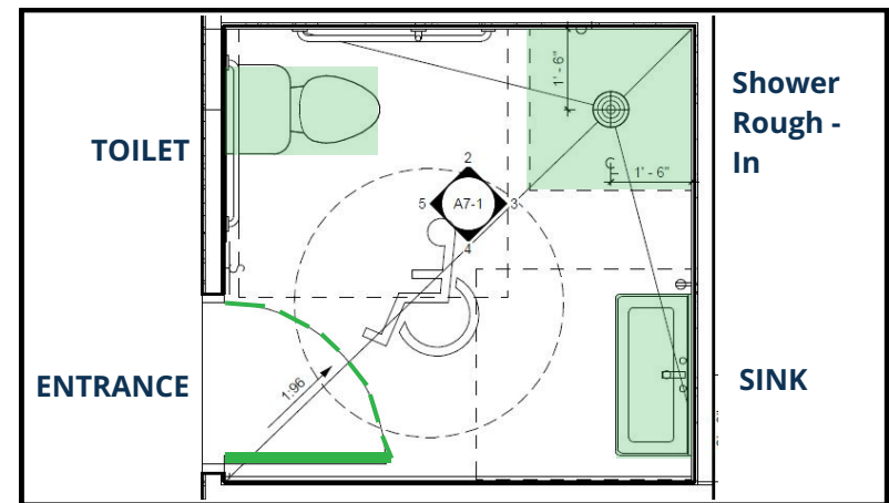
FLOOR PLAN
