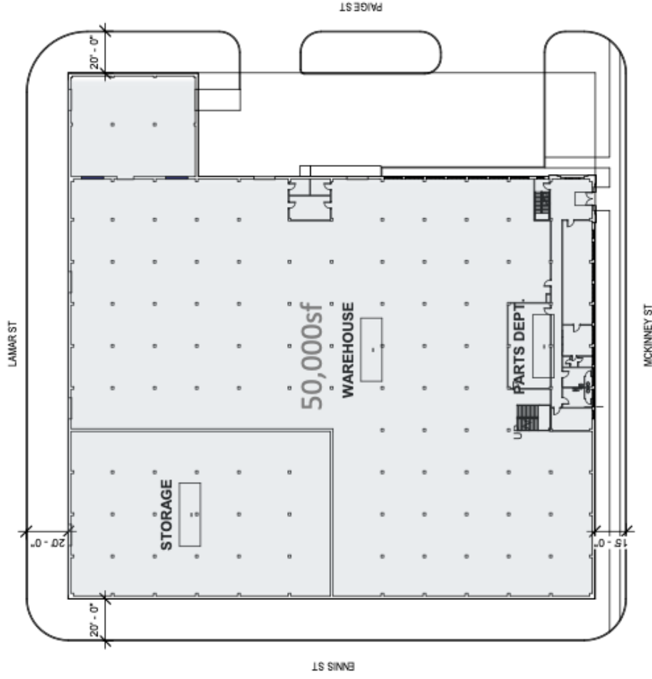
1 Level 1 1" = 40'-0"
