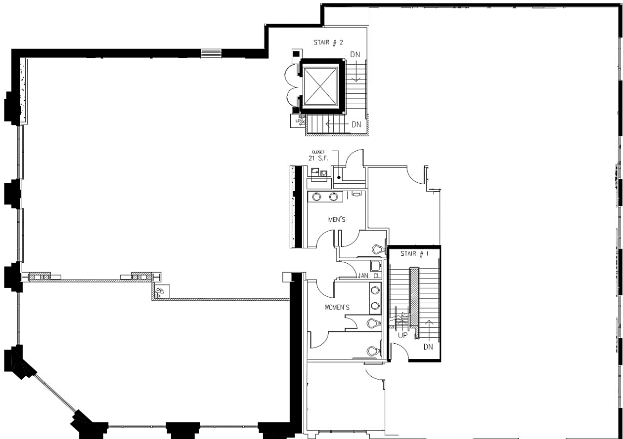
SECOND FLOOR SPACE PLAN
