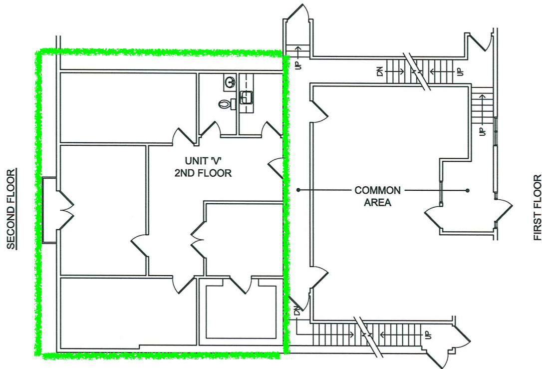
1 A200 EXISTING FLOOR PLAN SCALE: 1/8" = 1'-0"
