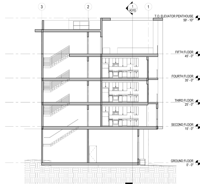
2 EAST/WEST BUILDING SECTION A310 1/8" = 1'-0"
