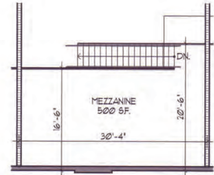
Mezz. Plan Type 'C' N.T.S. (Typical all Buildings)
