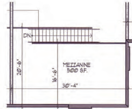
Mezz. Plan Type 'B' N.T.S. (Typical all Buildings)
