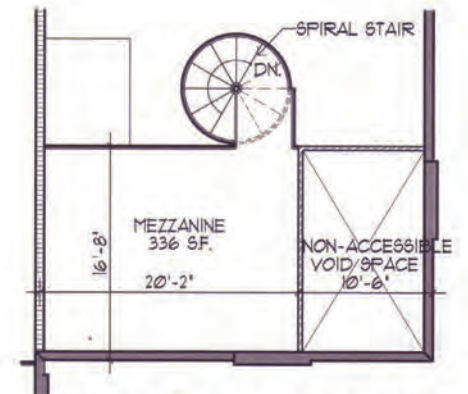
Mezz. Plan Type 'A' N.T.S. (Typical all Buildings)
