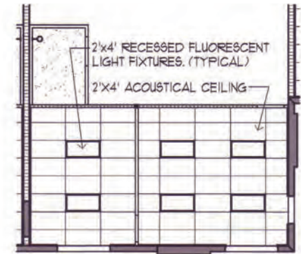
Reflected Ceiling Plan Type 'B' N.T.S. (Typical all Buildings)
