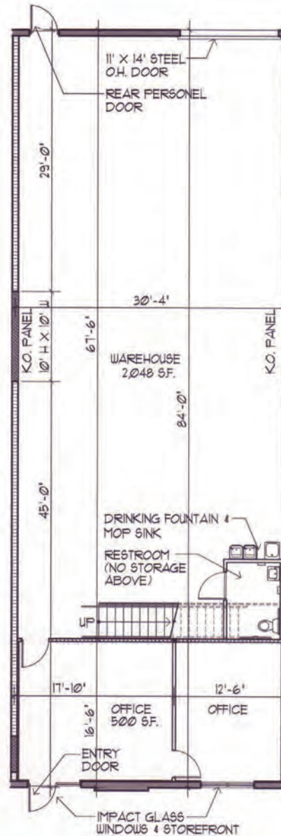
Bay Plan Type 'C' N.T.S. (Typical all Buildings)
