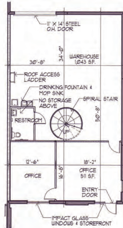
Bay Plan Type 'A' N.T.S. (Typical all Buildings)
