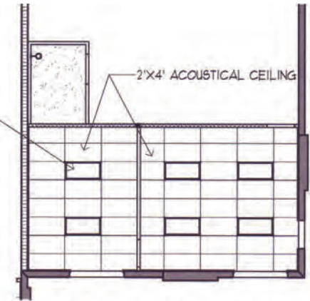
Reflected Ceiling Plan Type 'A' N.T.S. (Typical all Buildings)
