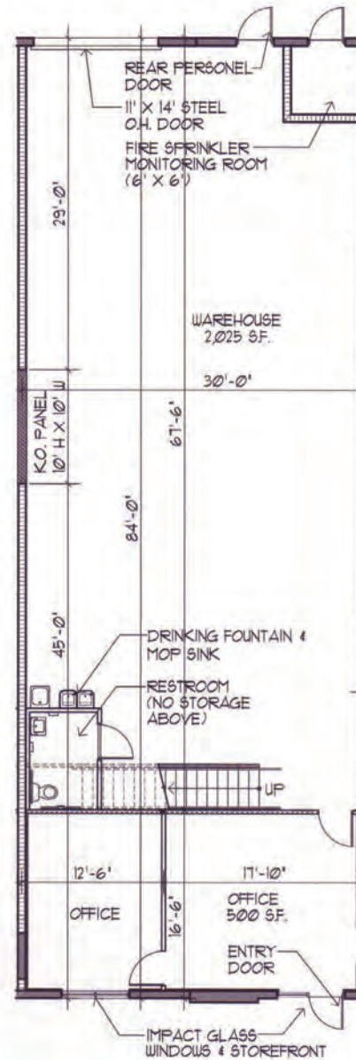
Bay Plan Type 'B' N.T.S. (Typical all Buildings)
