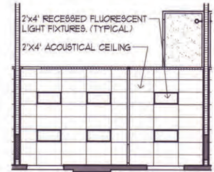
Reflected Ceiling Plan Type 'C' N.T.S. (Typical all Buildings)
