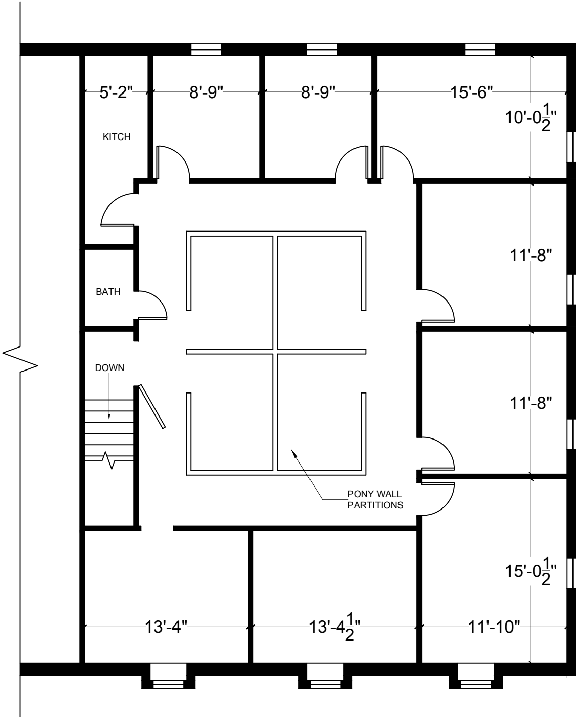
124 MINE LAKE : SECOND FLOOR scale: 1/8"=1'0"
