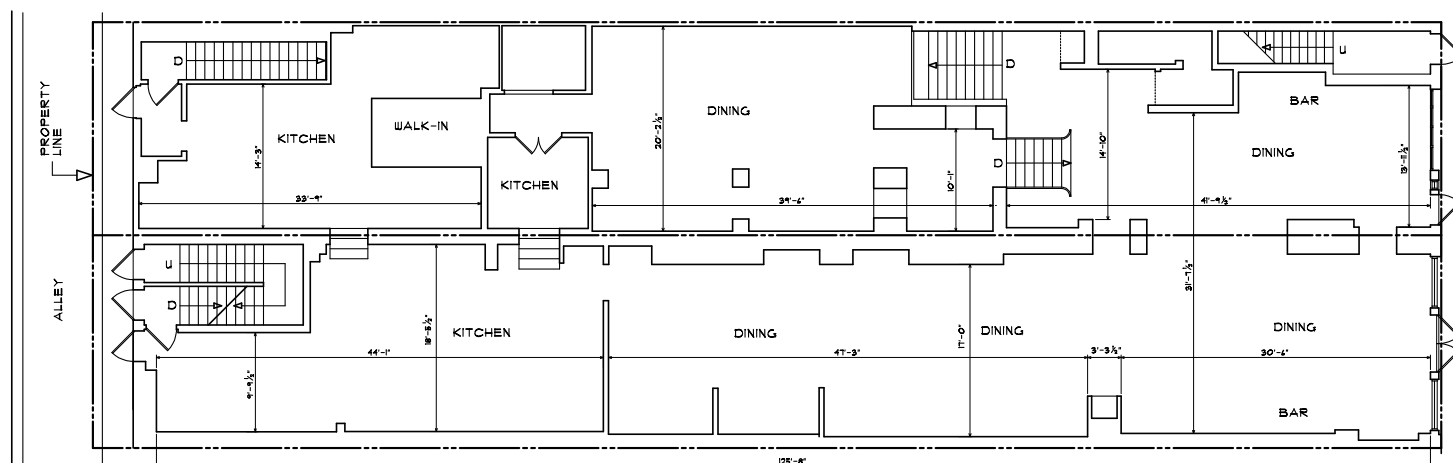
FIRST FLOOR PLAN NOTE: DIMENSIONS MAY VARY IN FIELD. 3/16"=1'-0"
