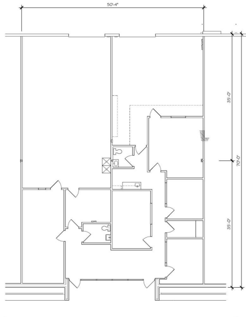
FLOOR PLAN -3464 sq.ft. 401 ISOM RD. suite #430
