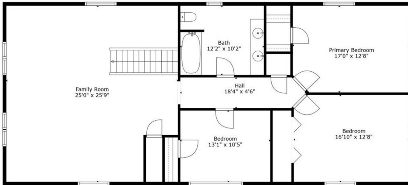
UPPER LEVEL
