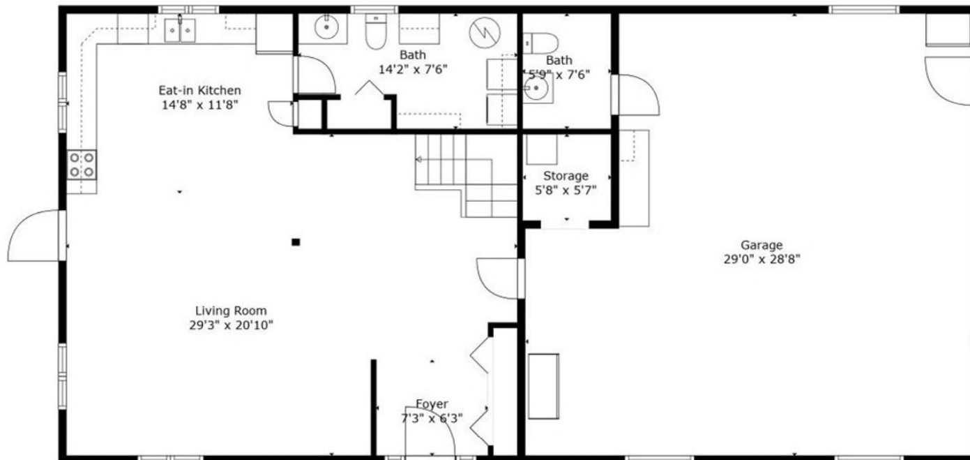
MAIN LEVEL
