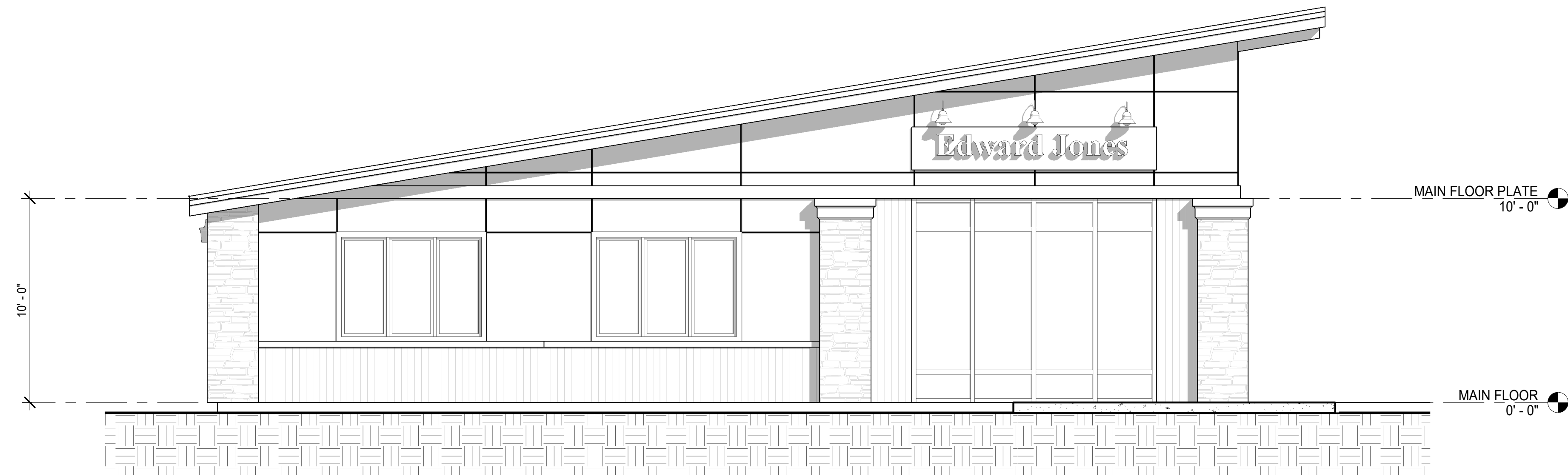
1 WEST ELEVATION 1/4" = 1'-0"
