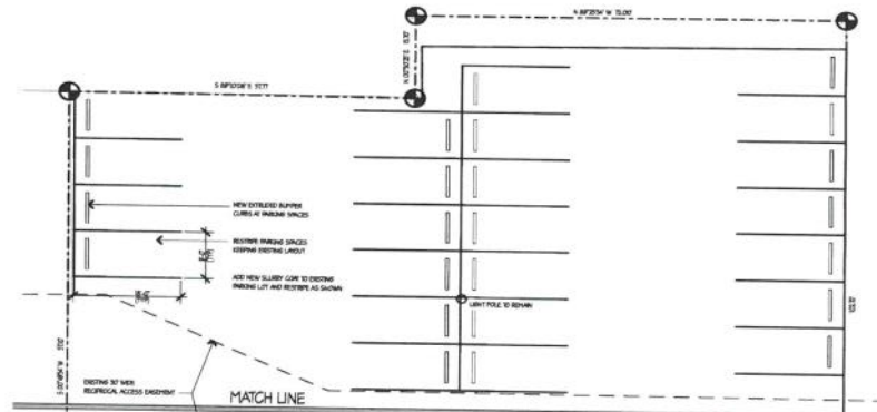
SITE PLAN - NORTH PORTION SCALE: 1" = 10'
