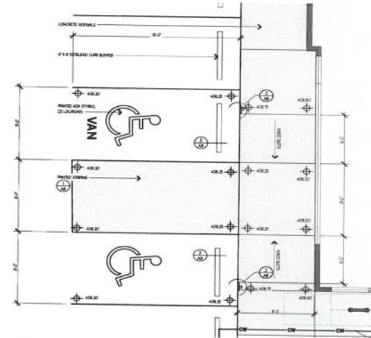
ENLARGED ADA PARKING SCALE: 1/4" = 1'-0"
