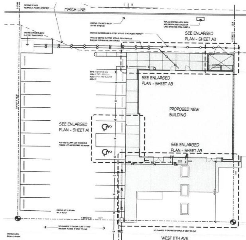
SITE PLAN - SOUTH PORTION SCALE: 1" = 10'
