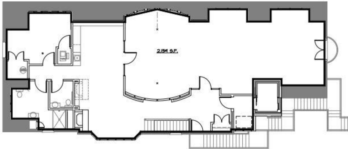
15 THIRD FLOOR FINISHES AND ELECTRICAL PLAN SCALE 1/4" = 1'-0"
