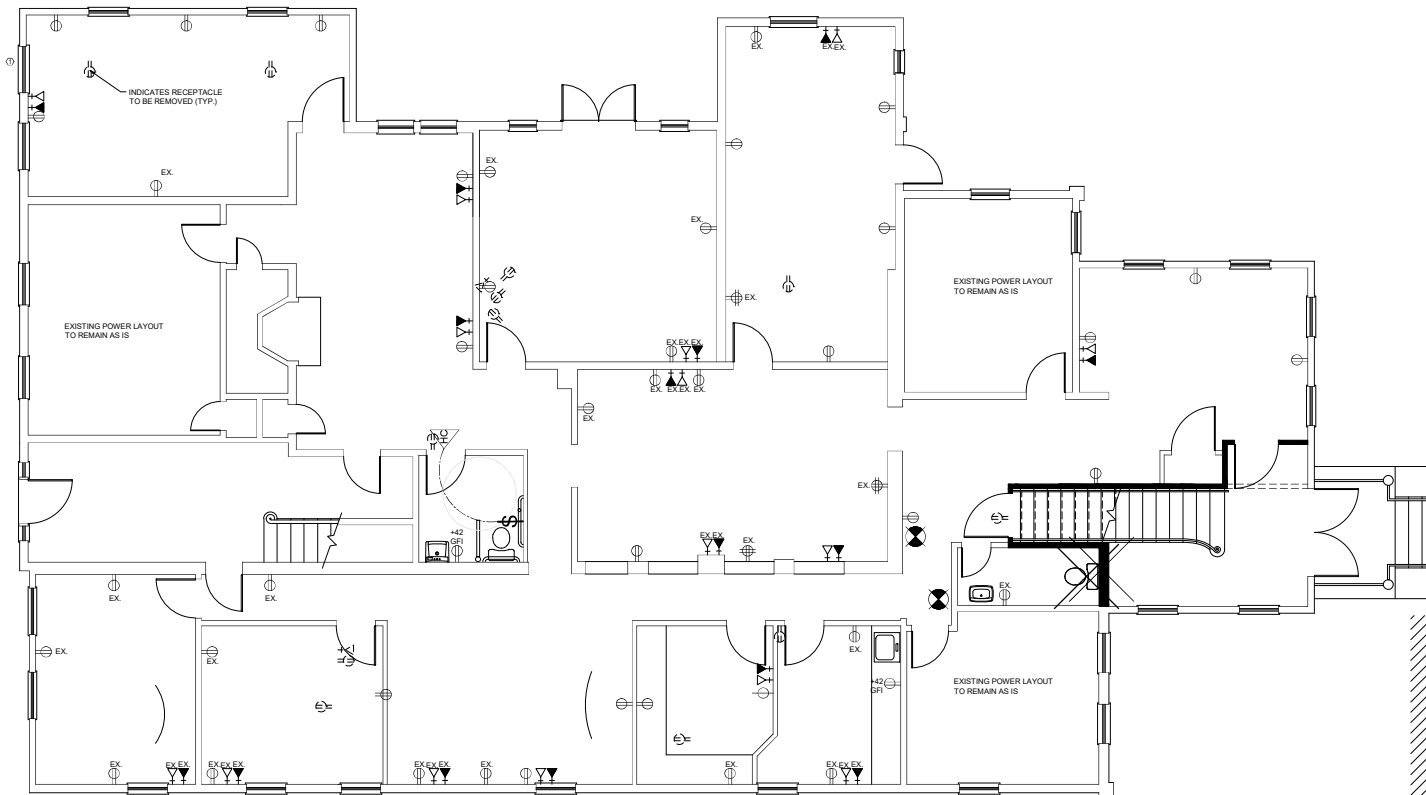
1 E1 FIRST FLOOR POWER PLAN SCALE: 1/4" = 1'-0"
