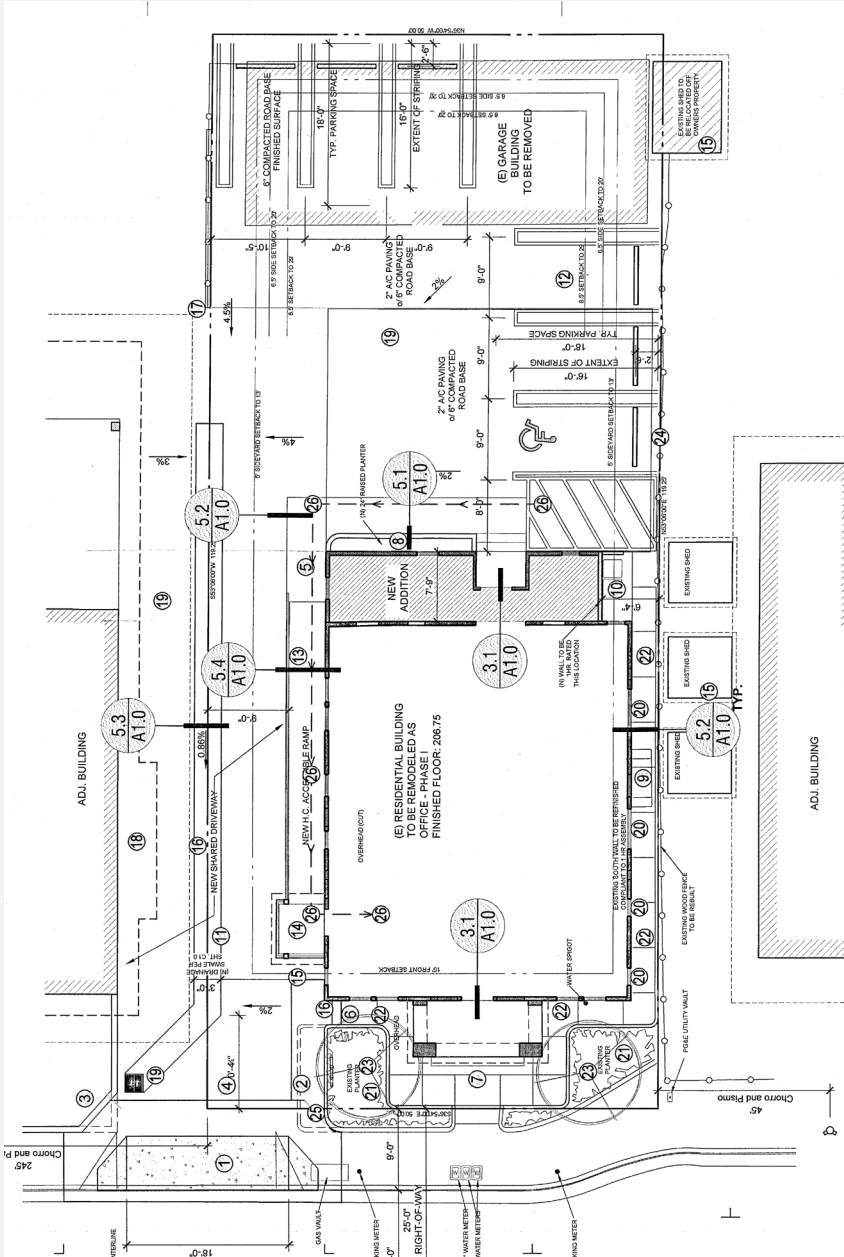
Site Plan
