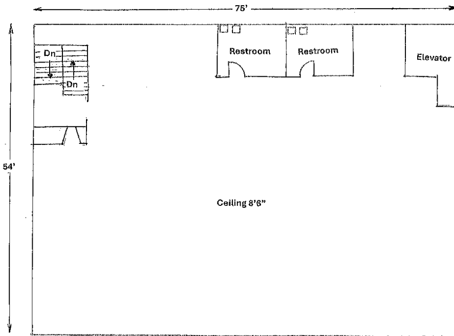
MEZZANINE 4,050 sq. ft.
