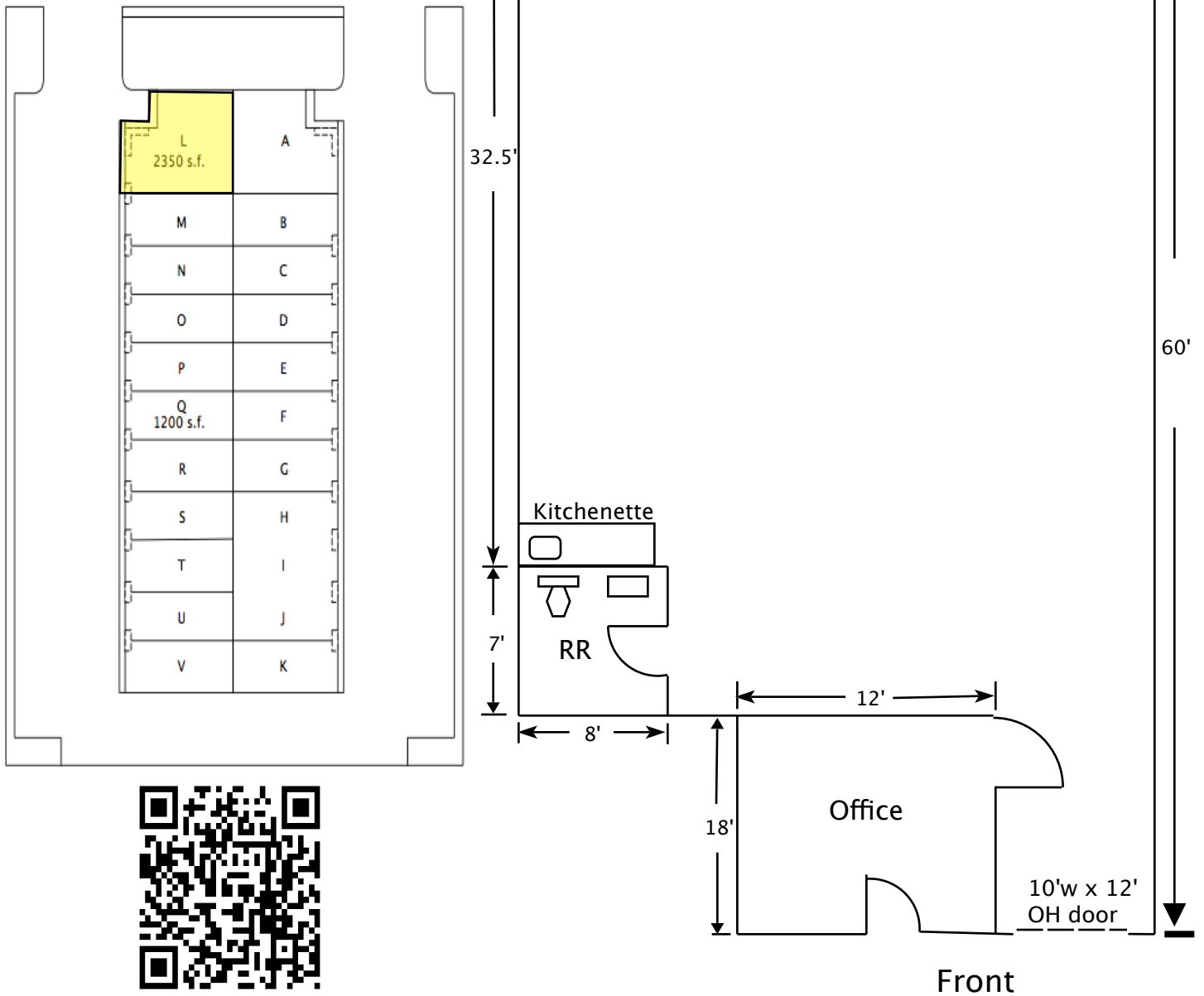
VERNON BUSINESS PARK SITE PLAN
