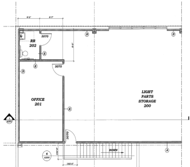
4 FLOOR PLAN SCALE 1/4"=1'-0"
