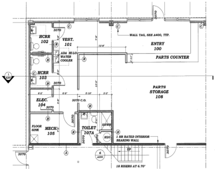
3 FLOOR PLAN SCALE 1/4"=1'-0"
