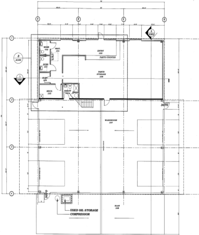
1 FLOOR PLAN SCALE 1/4"=1'-0"
