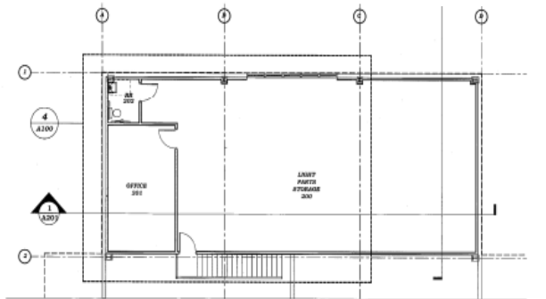
1 SECOND FLOOR SCALE 1/4"=1'-0"
