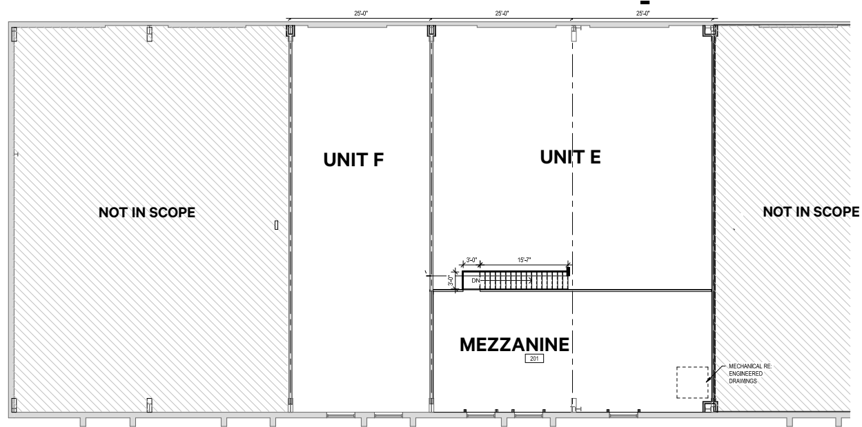
SECOND FLOOR MEZZANINE
