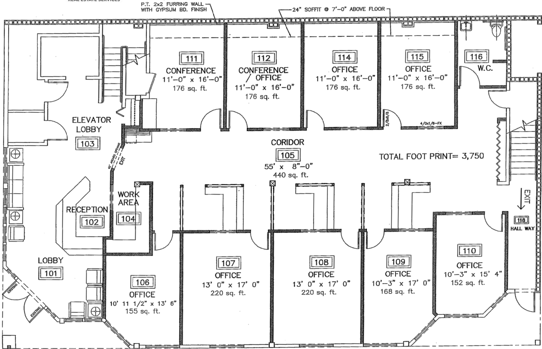
1 First FLOOR PLAN 1 SCALE: 1/8" = 1'-0"
