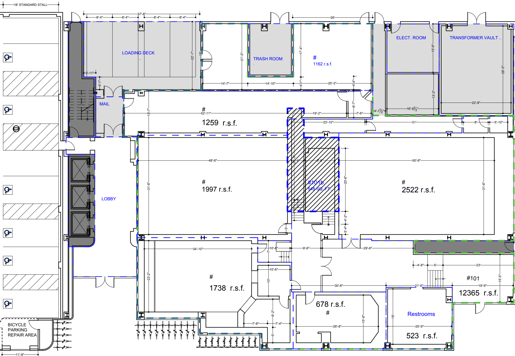
15' 0 15 30 1/16"=1'-0" 1st LEVEL 1/16" = 1'-0" 04/02/20
