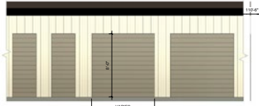
3 TYP TRADITIONAL STORAGE INTERIOR ELEVATION w/ DOORS 1/8" = 1'-0"
