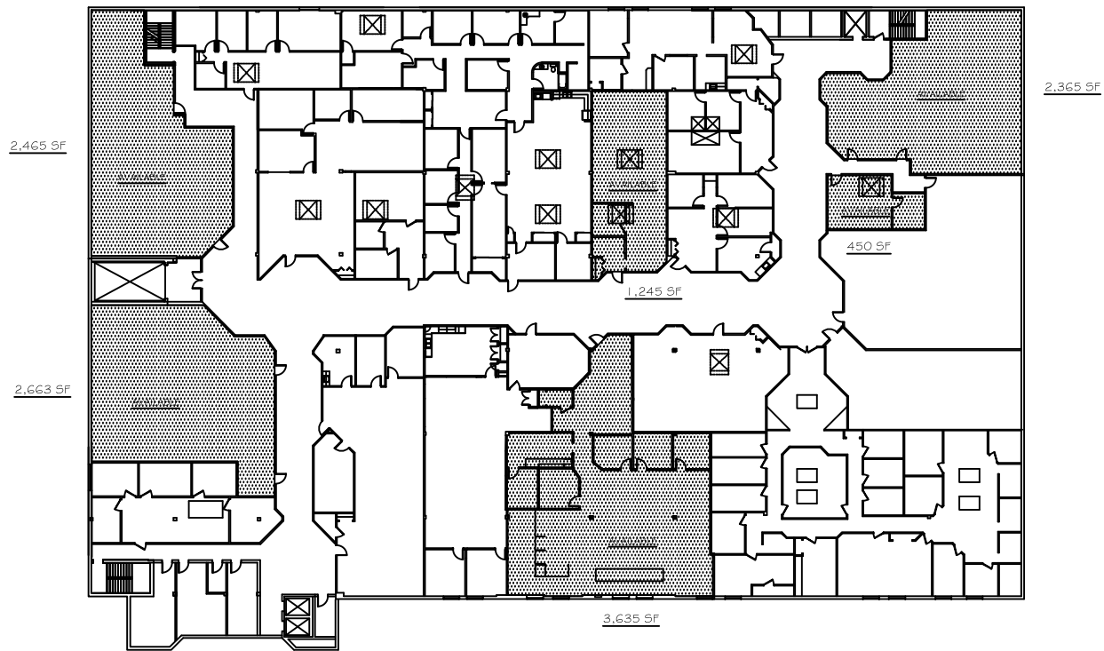
1 THIRD FLOOR PLAN 1/32"=1'-0"
