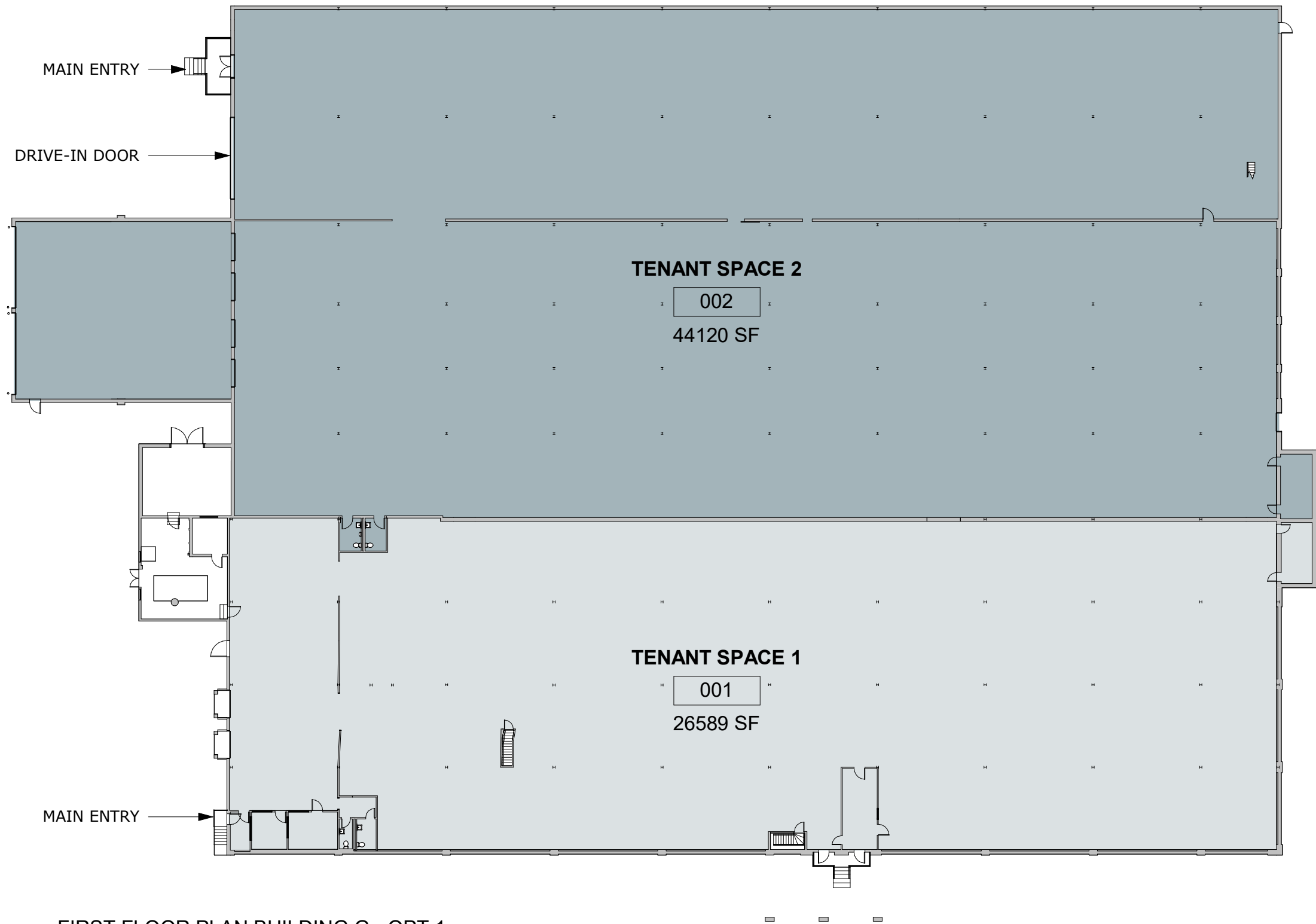
① FIRST FLOOR PLAN BUILDING G - OPT 1 1/32" = 1'-0"
