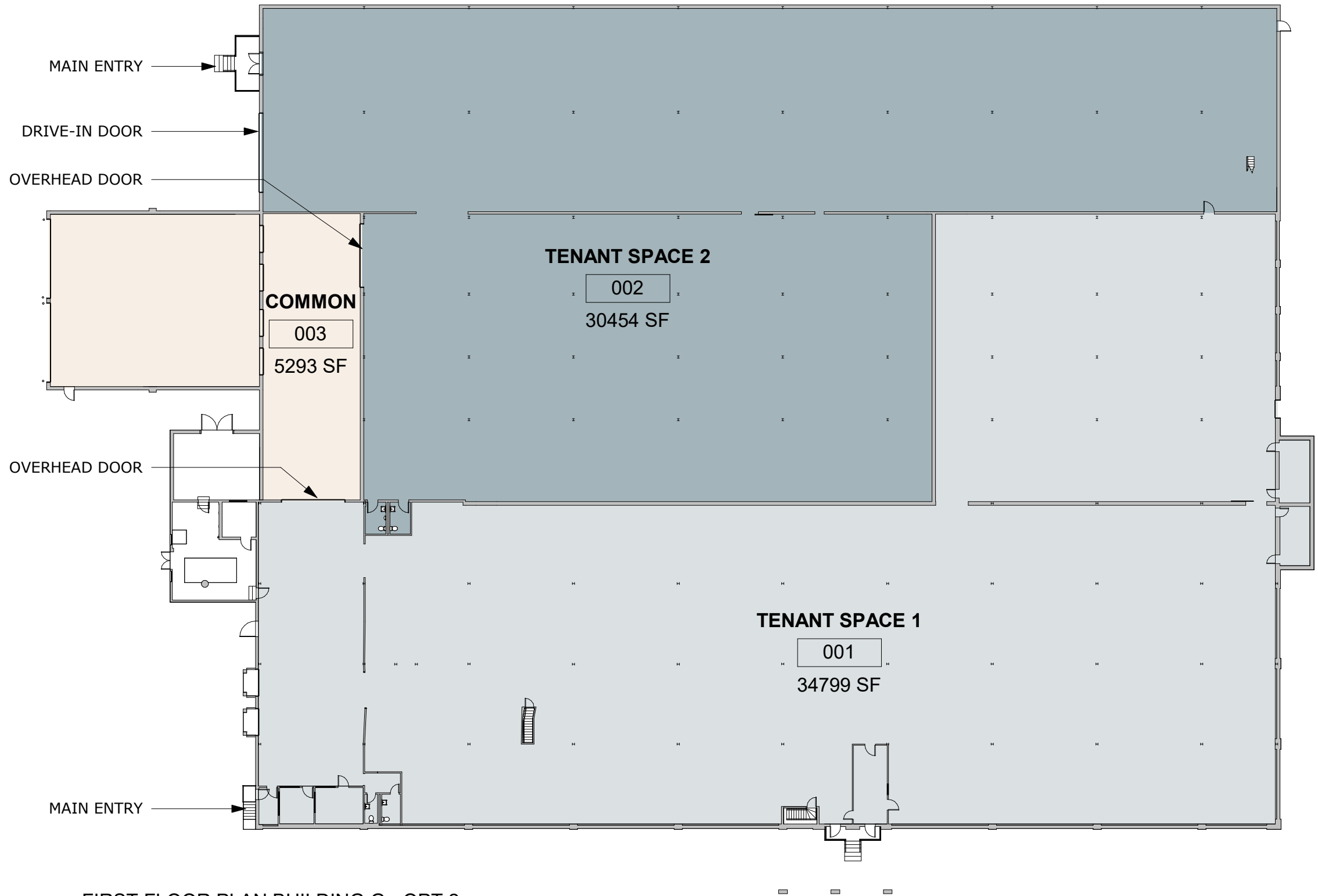
1 FIRST FLOOR PLAN BUILDING G - OPT 2 1/32" = 1'-0"
