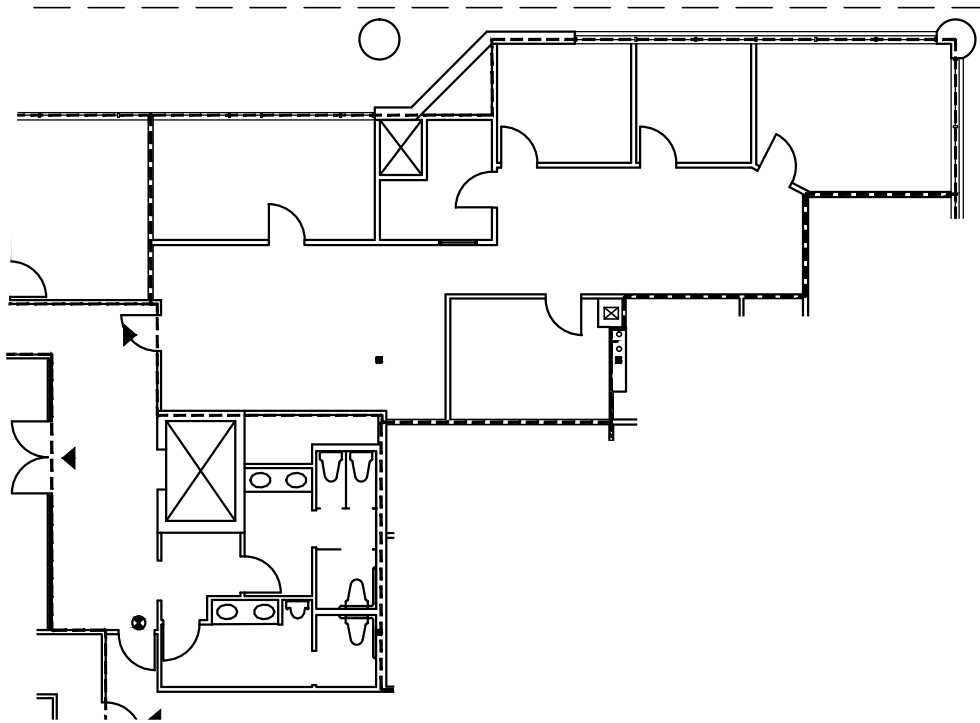
① FOURTH FLOOR PLAN—SUITE 402 SCALE 1"=16'-0"
