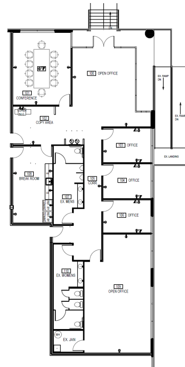
Suite A new office demo/plan
