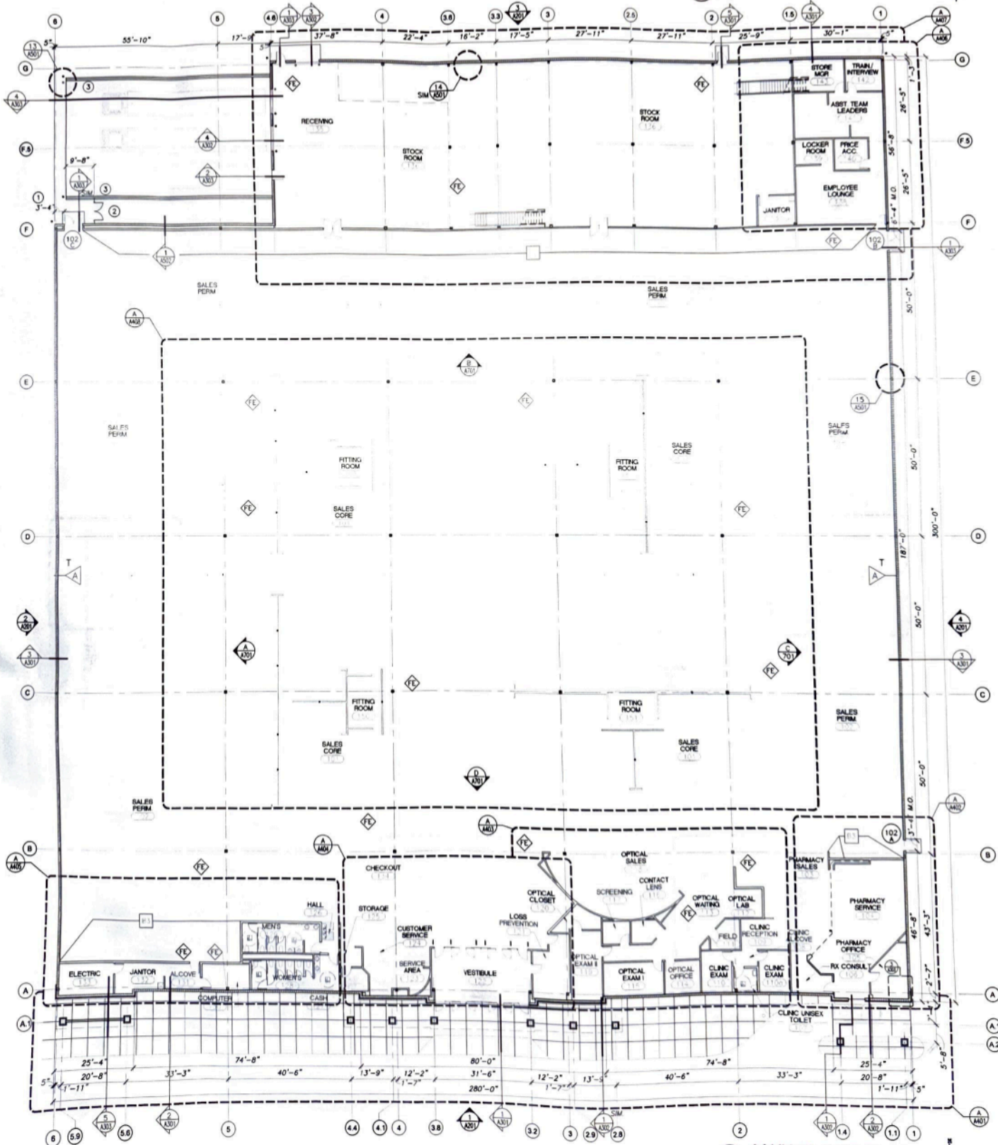
1 MAIN FLOOR PLAN A101 1/16" = 1'-0"
