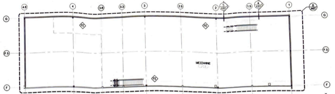
2 MEZZANINE FLOOR PLAN A101 1/16" = 1'-0"
