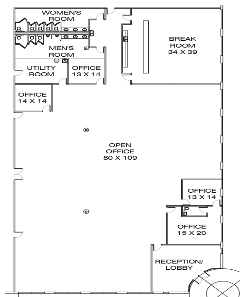
NORTH OFFICE FLOOR PLAN
