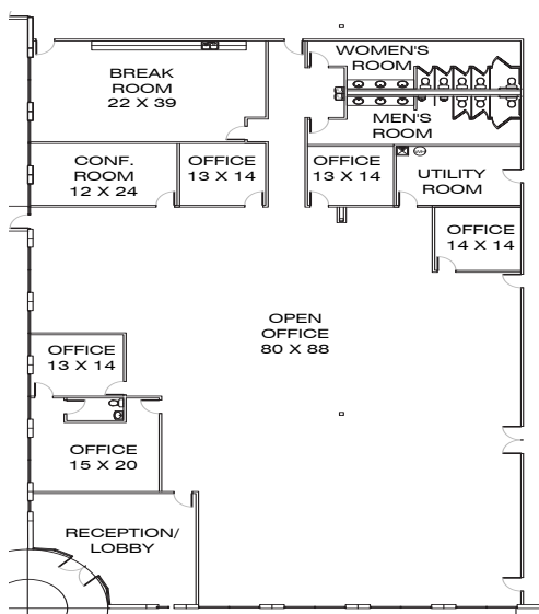
SOUTH OFFICE FLOOR PLAN
