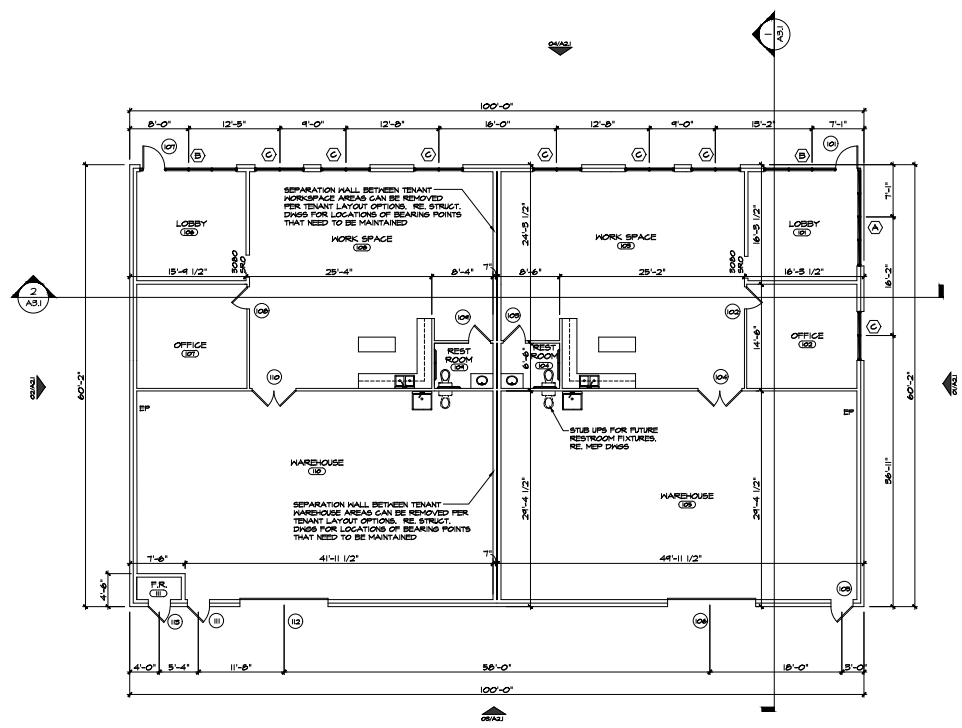
01 - FLOOR PLAN
