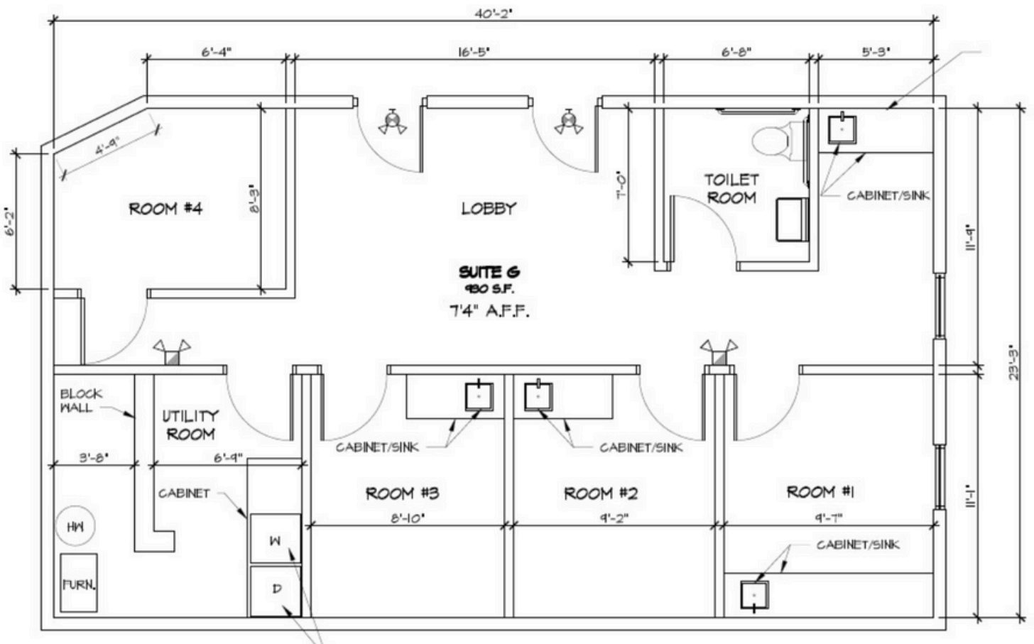
FLOOR PLAN
