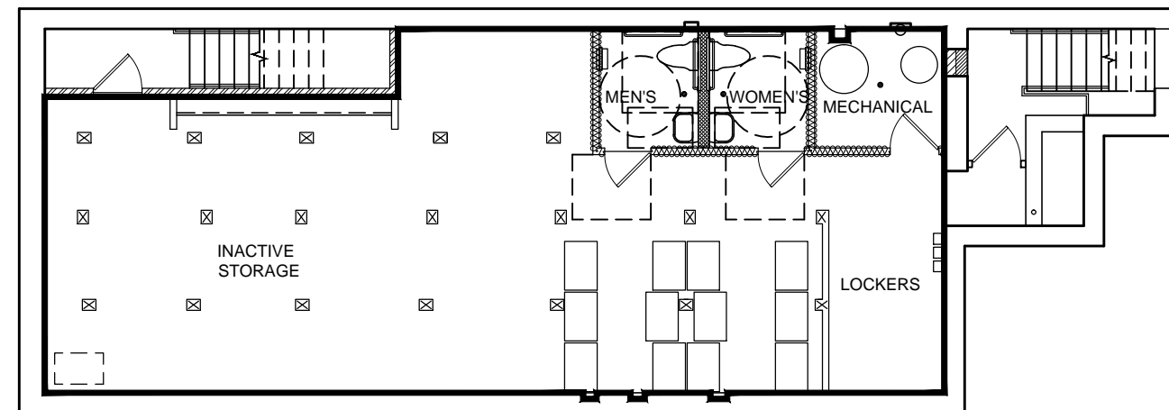
2 1.0 BASEMENT FLOOR PLAN SCALE: \frac{3}{32}'' = 1'-0''
