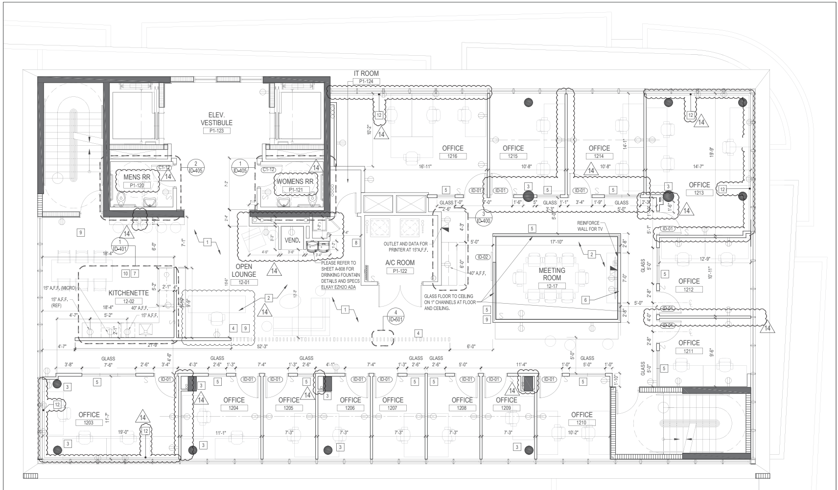
01 LEVEL 12 - INTERIOR LAYOUT
