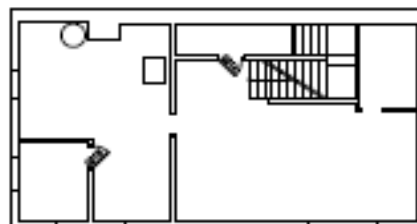
BASEMENT LEVEL EXISTING CONDITIONS FLOOR PLAN
