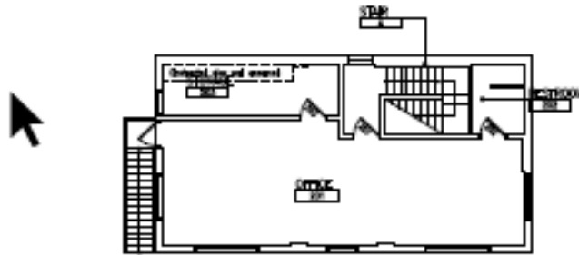
UPPER LEVEL EXISTING CONDITIONS FLOOR PLAN
