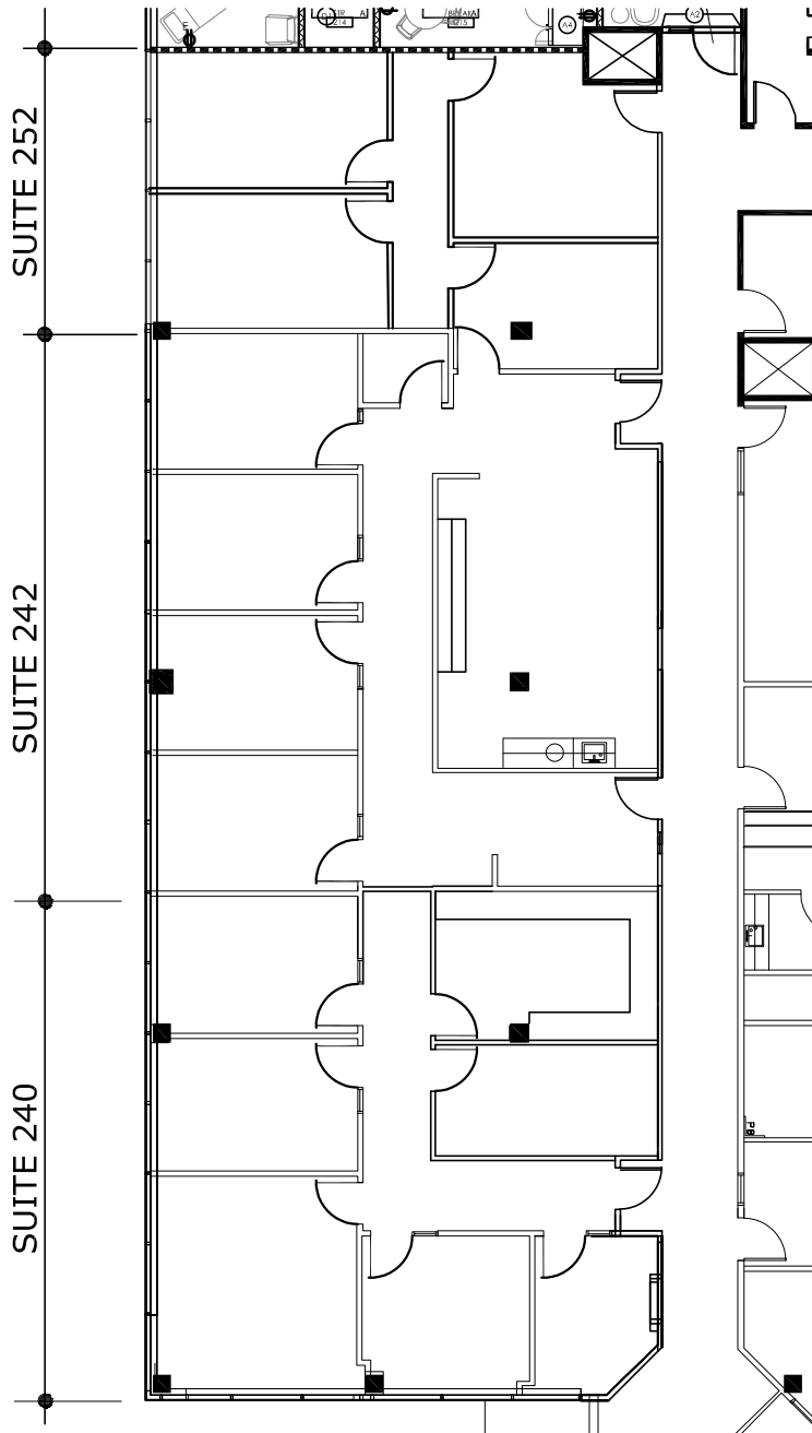
EXISTING PLAN:
