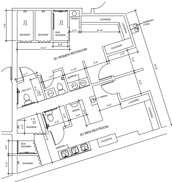
ENLARGED PLAN OF EXISTING RESTROOMS
