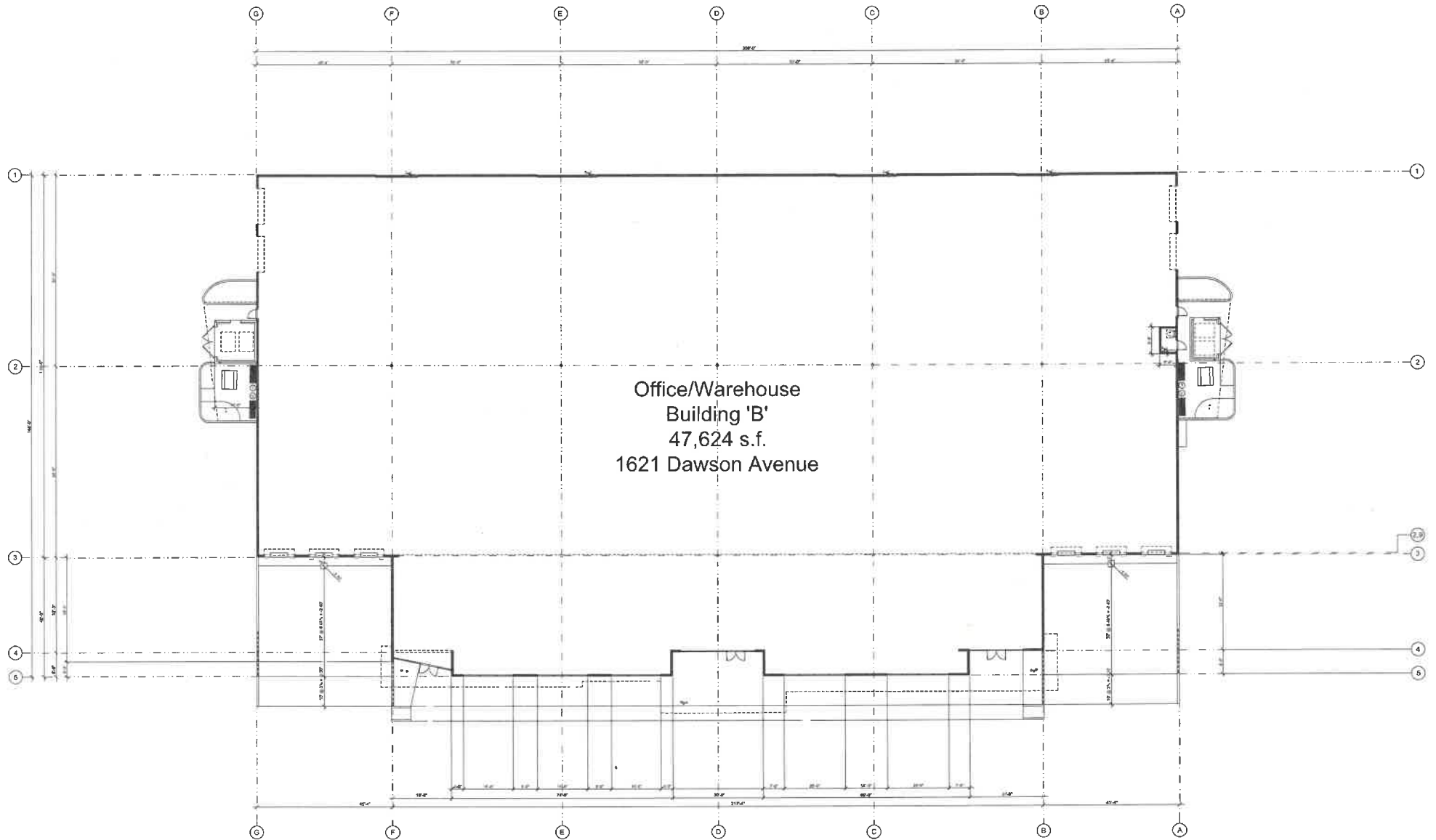
1 Floor Plan - Building 'B'
