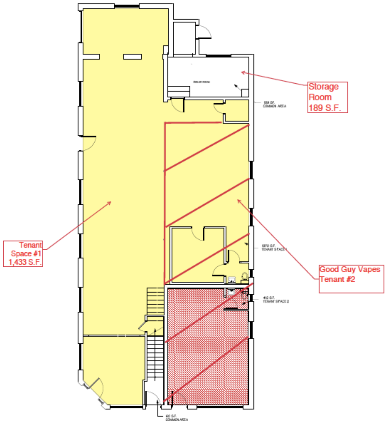
1 FIRST FLOOR PLAN SCALE: 3/8" = 1'-0"
