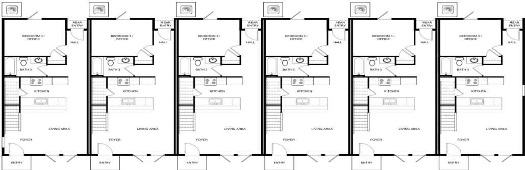
GROUND LEVEL OVERALL BUILDING PLAN
